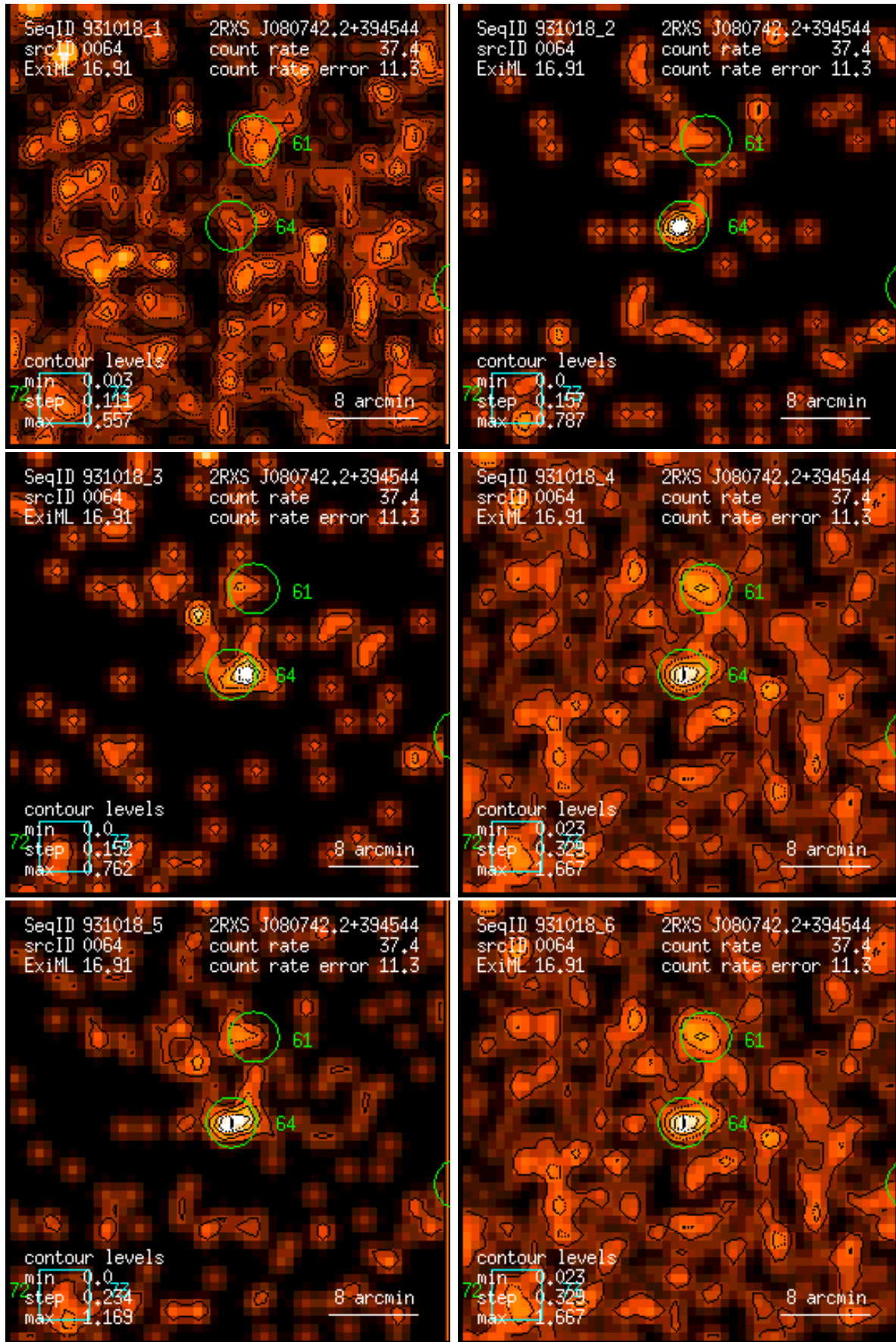
Figure 64: RASS 931018: detection 0064: band rate images, Gaussian filter: (1) PSPC channels 11 – 41, (2) 52 – 90, (3) 91 – 201, (4) 11 – 235, (5) 52 – 201, (6) 11 – 201. Broad band rates in counts/ks. Band rate contour levels in counts/ks/arcmin 2 .
