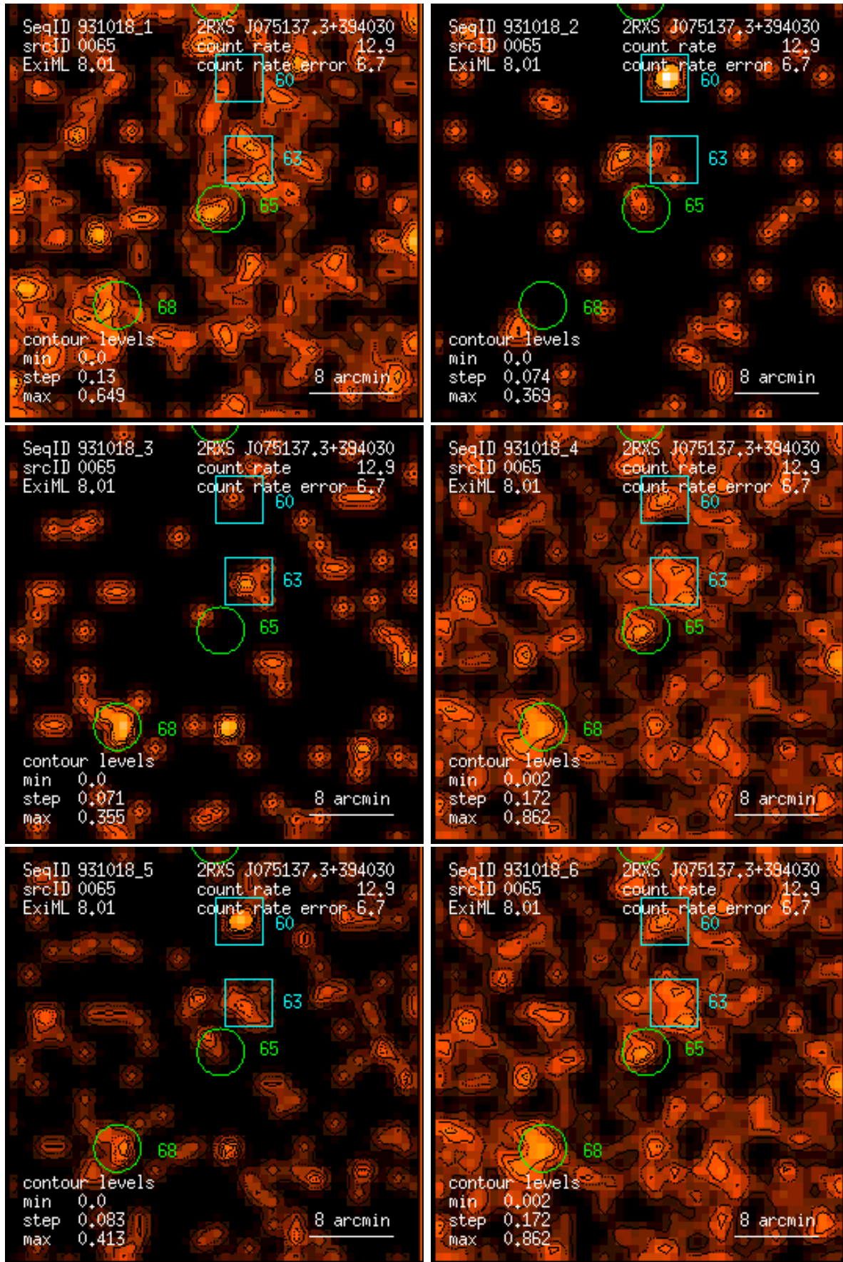
Figure 65: RASS 931018: detection 0065: band rate images, Gaussian filter: (1) PSPC channels 11 – 41, (2) 52 – 90, (3) 91 – 201, (4) 11 – 235, (5) 52 – 201, (6) 11 – 201. Broad band rates in counts/ks. Band rate contour levels in counts/ks/arcmin 2 .
