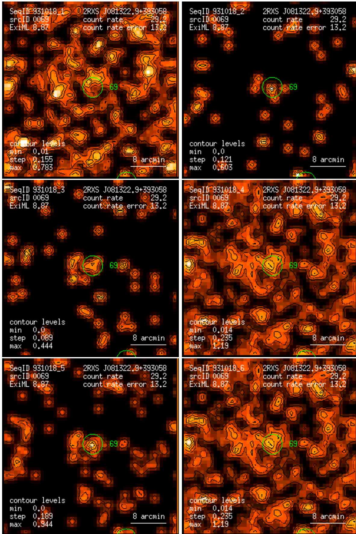
Figure 69: RASS 931018: detection 0069: band rate images, Gaussian filter: (1) PSPC channels 11 – 41, (2) 52 – 90, (3) 91 – 201, (4) 11 – 235, (5) 52 – 201, (6) 11 – 201. Broad band rates in counts/ks. Band rate contour levels in counts/ks/arcmin 2 .
