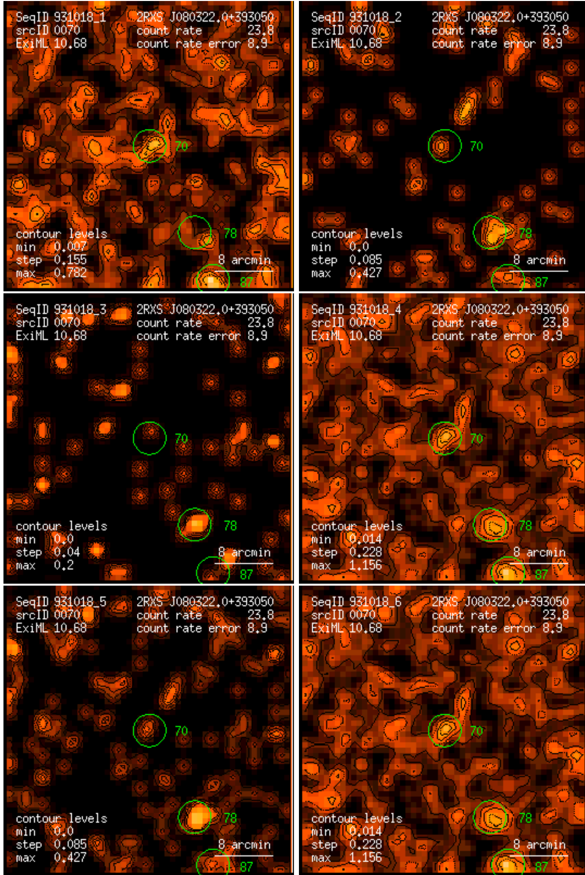
Figure 70: RASS 931018: detection 0070: band rate images, Gaussian filter: (1) PSPC channels 11 – 41, (2) 52 – 90, (3) 91 – 201, (4) 11 – 235, (5) 52 – 201, (6) 11 – 201. Broad band rates in counts/ks. Band rate contour levels in counts/ks/arcmin 2 .
