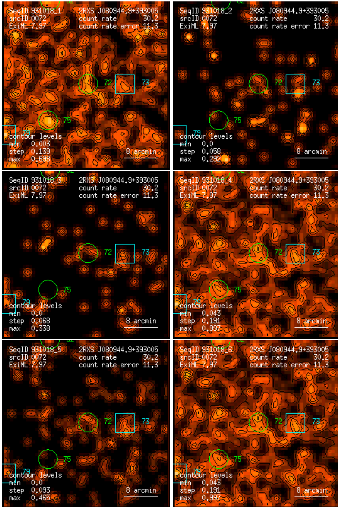
Figure 72: RASS 931018: detection 0072: band rate images, Gaussian filter: (1) PSPC channels 11 – 41, (2) 52 – 90, (3) 91 – 201, (4) 11 – 235, (5) 52 – 201, (6) 11 – 201. Broad band rates in counts/ks. Band rate contour levels in counts/ks/arcmin 2 .
