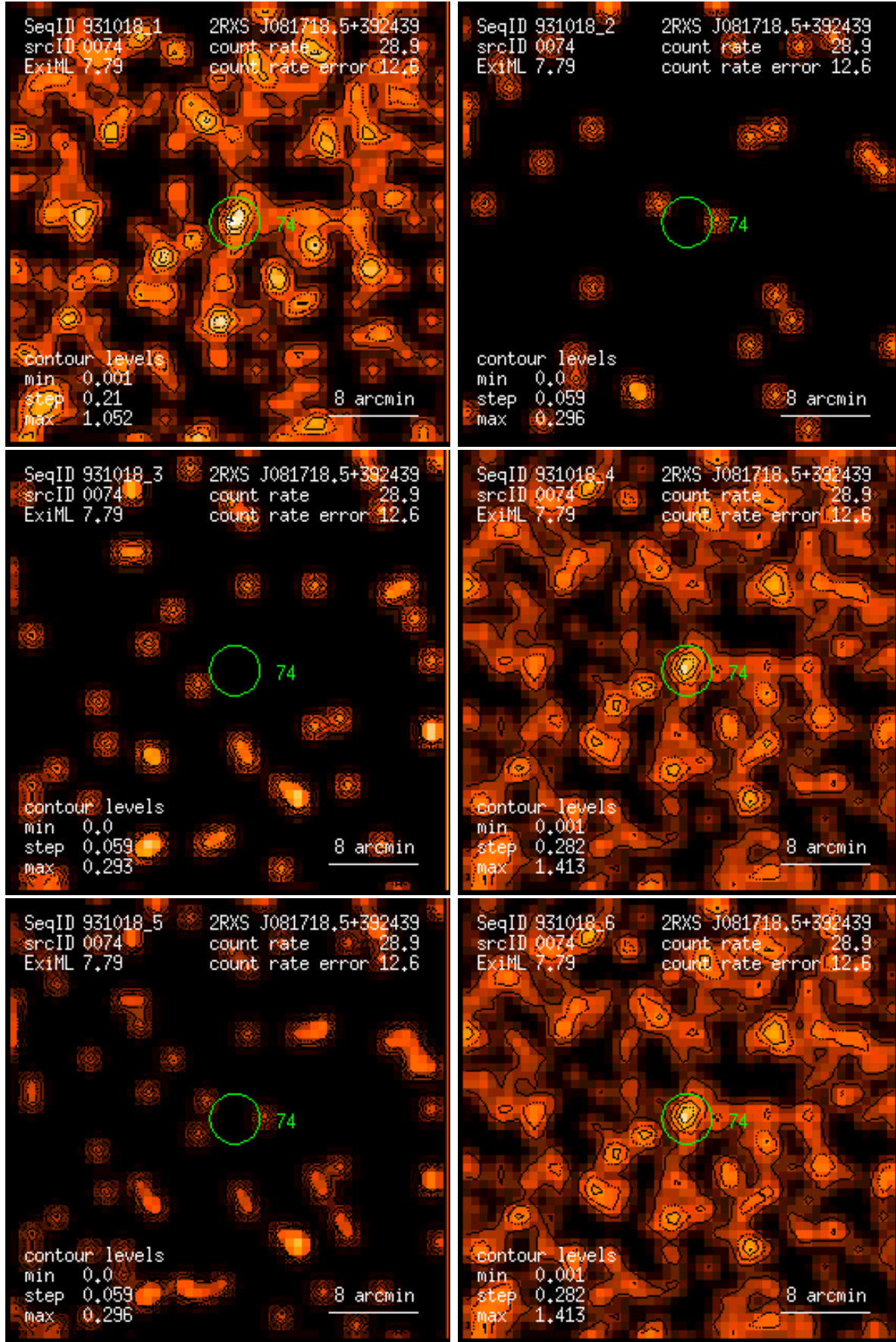
Figure 74: RASS 931018: detection 0074: band rate images, Gaussian filter: (1) PSPC channels 11 – 41, (2) 52 – 90, (3) 91 – 201, (4) 11 – 235, (5) 52 – 201, (6) 11 – 201. Broad band rates in counts/ks. Band rate contour levels in counts/ks/arcmin 2 .
