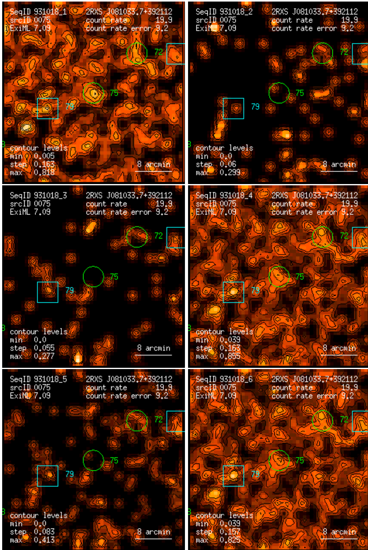
Figure 75: RASS 931018: detection 0075: band rate images, Gaussian filter: (1) PSPC channels 11 – 41, (2) 52 – 90, (3) 91 – 201, (4) 11 – 235, (5) 52 – 201, (6) 11 – 201. Broad band rates in counts/ks. Band rate contour levels in counts/ks/arcmin 2 .
