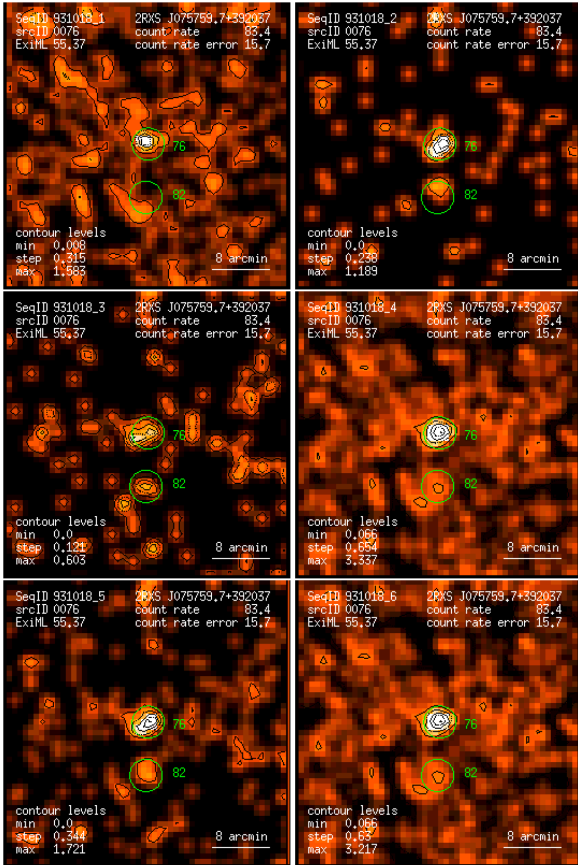
Figure 76: RASS 931018: detection 0076: band rate images, Gaussian filter: (1) PSPC channels 11 – 41, (2) 52 – 90, (3) 91 – 201, (4) 11 – 235, (5) 52 – 201, (6) 11 – 201. Broad band rates in counts/ks. Band rate contour levels in counts/ks/arcmin 2 .
