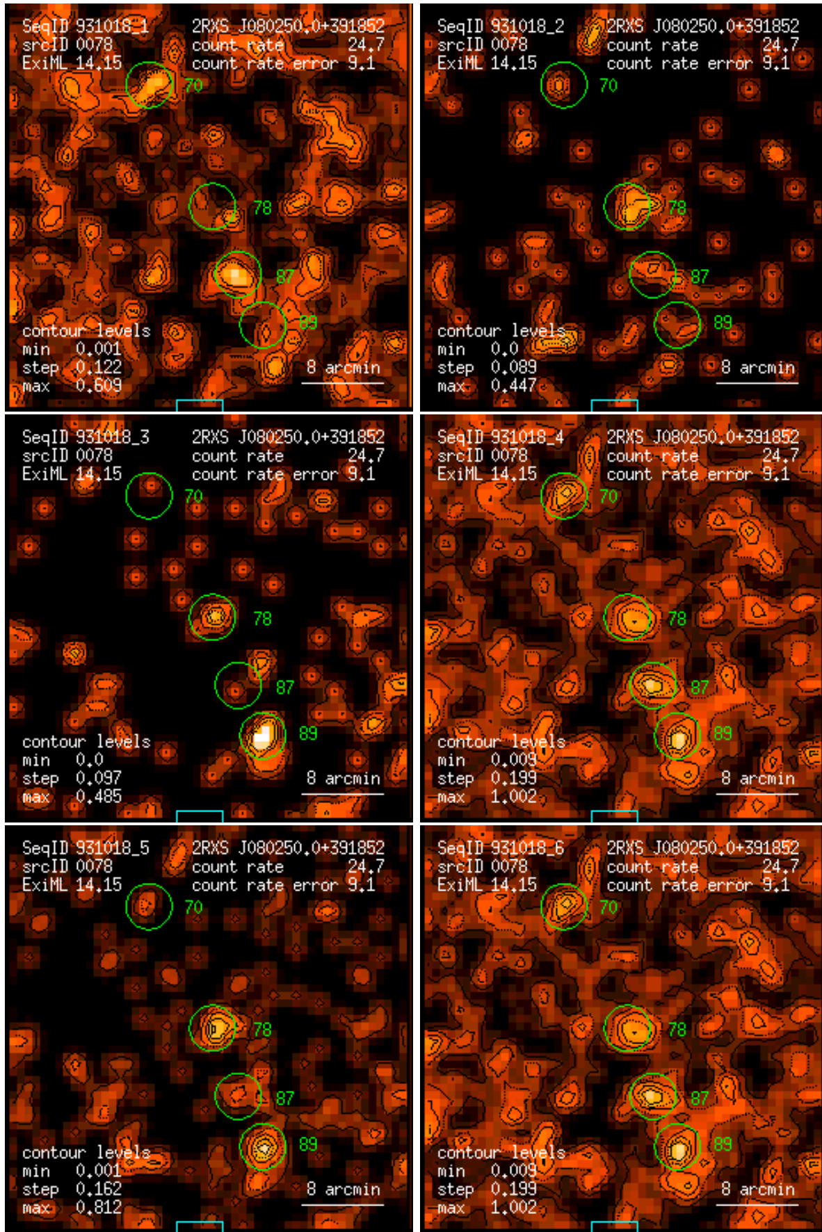
Figure 78: RASS 931018: detection 0078: band rate images, Gaussian filter: (1) PSPC channels 11 – 41, (2) 52 – 90, (3) 91 – 201, (4) 11 – 235, (5) 52 – 201, (6) 11 – 201. Broad band rates in counts/ks. Band rate contour levels in counts/ks/arcmin 2 .
