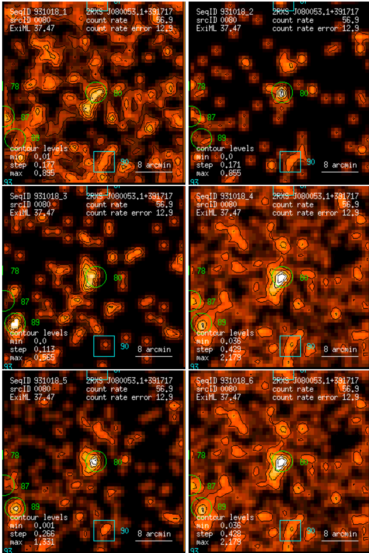
Figure 80: RASS 931018: detection 0080: band rate images, Gaussian filter: (1) PSPC channels 11 – 41, (2) 52 – 90, (3) 91 – 201, (4) 11 – 235, (5) 52 – 201, (6) 11 – 201. Broad band rates in counts/ks. Band rate contour levels in counts/ks/arcmin 2 .
