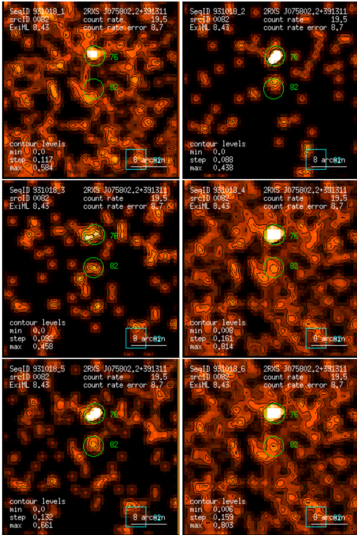
Figure 82: RASS 931018: detection 0082: band rate images, Gaussian filter: (1) PSPC channels 11 – 41, (2) 52 – 90, (3) 91 – 201, (4) 11 – 235, (5) 52 – 201, (6) 11 – 201. Broad band rates in counts/ks. Band rate contour levels in counts/ks/arcmin 2 .
