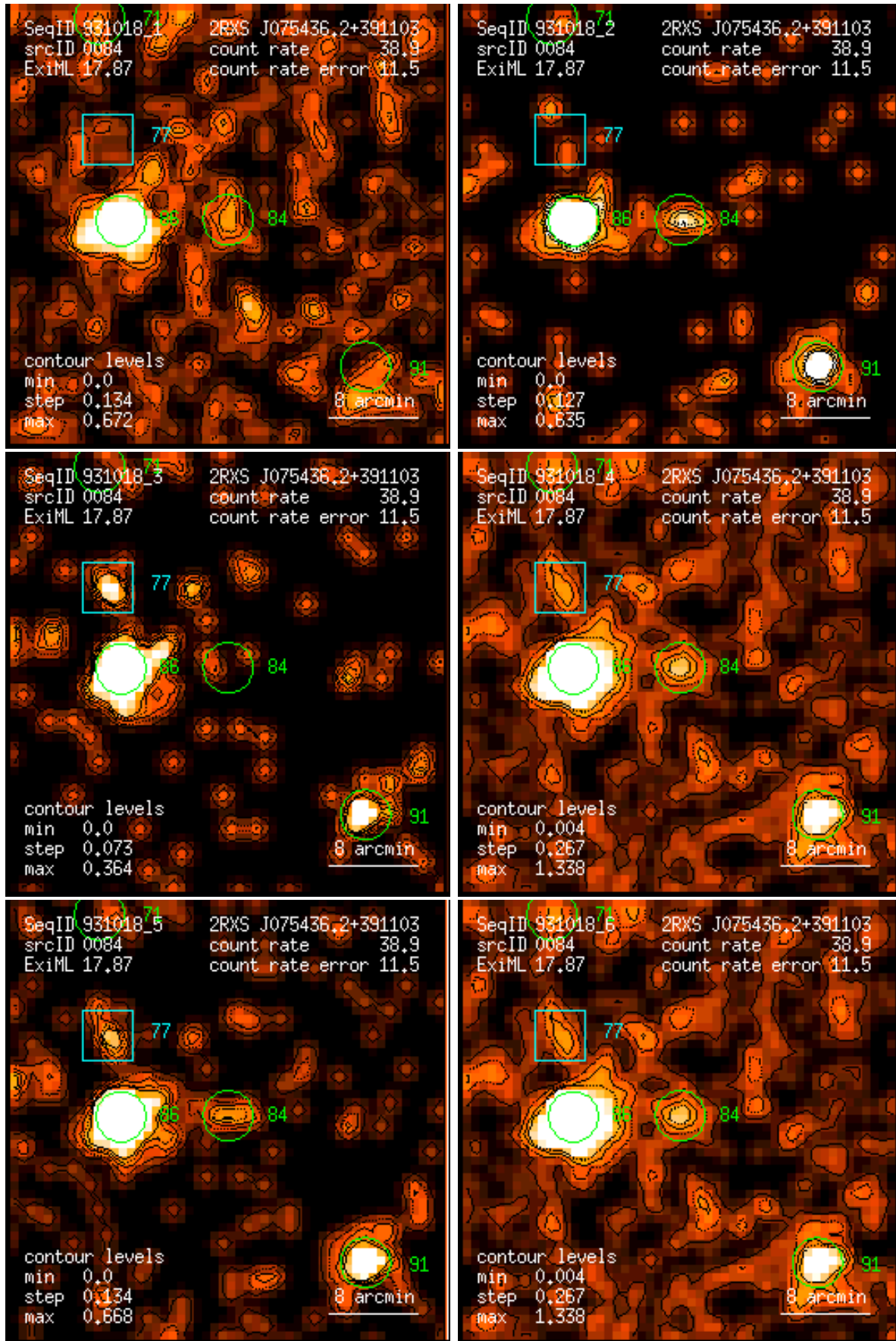
Figure 84: RASS 931018: detection 0084: band rate images, Gaussian filter: (1) PSPC channels 11 – 41, (2) 52 – 90, (3) 91 – 201, (4) 11 – 235, (5) 52 – 201, (6) 11 – 201. Broad band rates in counts/ks. Band rate contour levels in counts/ks/arcmin 2 .
