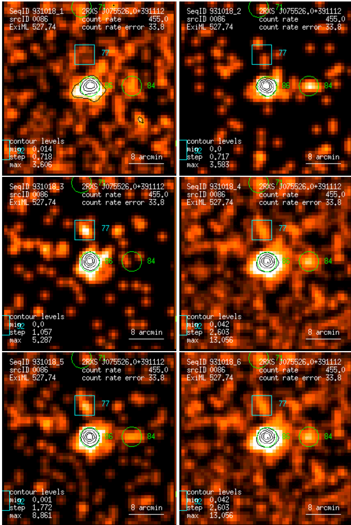
Figure 86: RASS 931018: detection 0086: band rate images, Gaussian filter: (1) PSPC channels 11 – 41, (2) 52 – 90, (3) 91 – 201, (4) 11 – 235, (5) 52 – 201, (6) 11 – 201. Broad band rates in counts/ks. Band rate contour levels in counts/ks/arcmin 2 .
