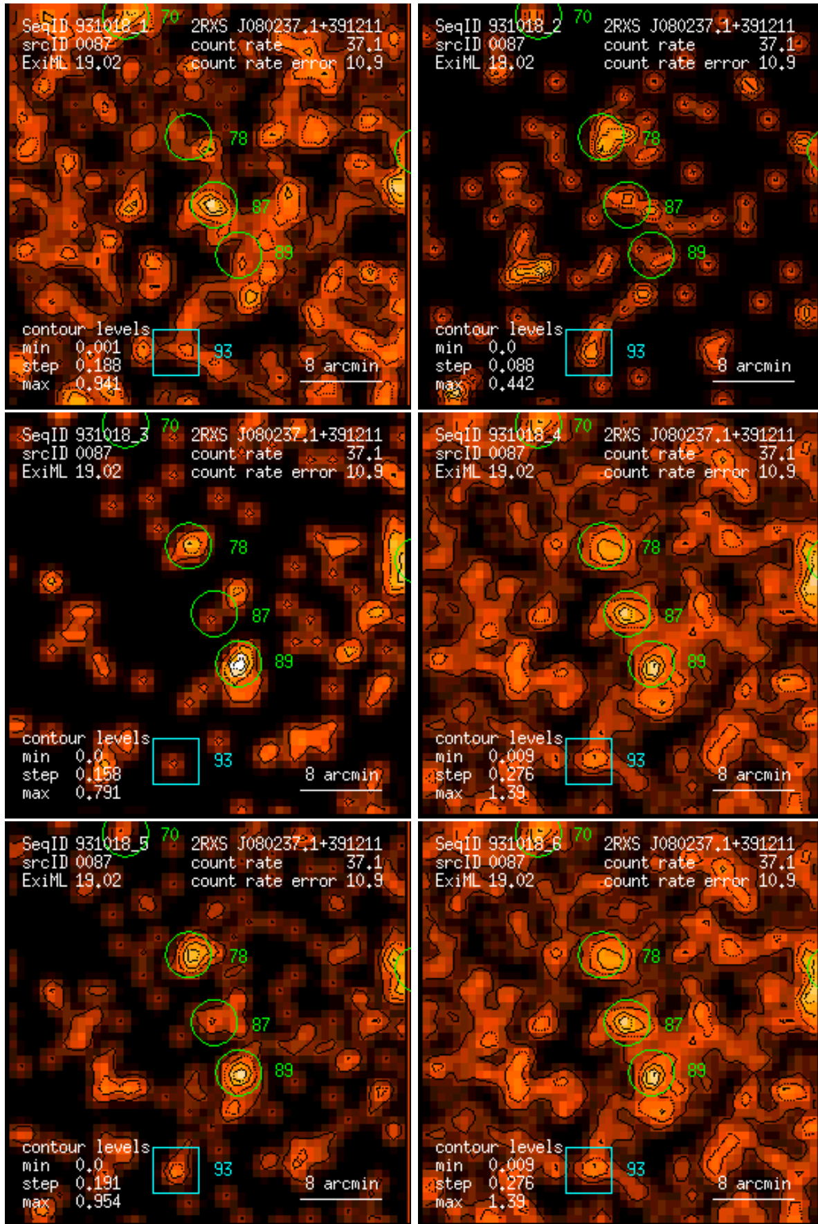
Figure 87: RASS 931018: detection 0087: band rate images, Gaussian filter: (1) PSPC channels 11 – 41, (2) 52 – 90, (3) 91 – 201, (4) 11 – 235, (5) 52 – 201, (6) 11 – 201. Broad band rates in counts/ks. Band rate contour levels in counts/ks/arcmin 2 .
