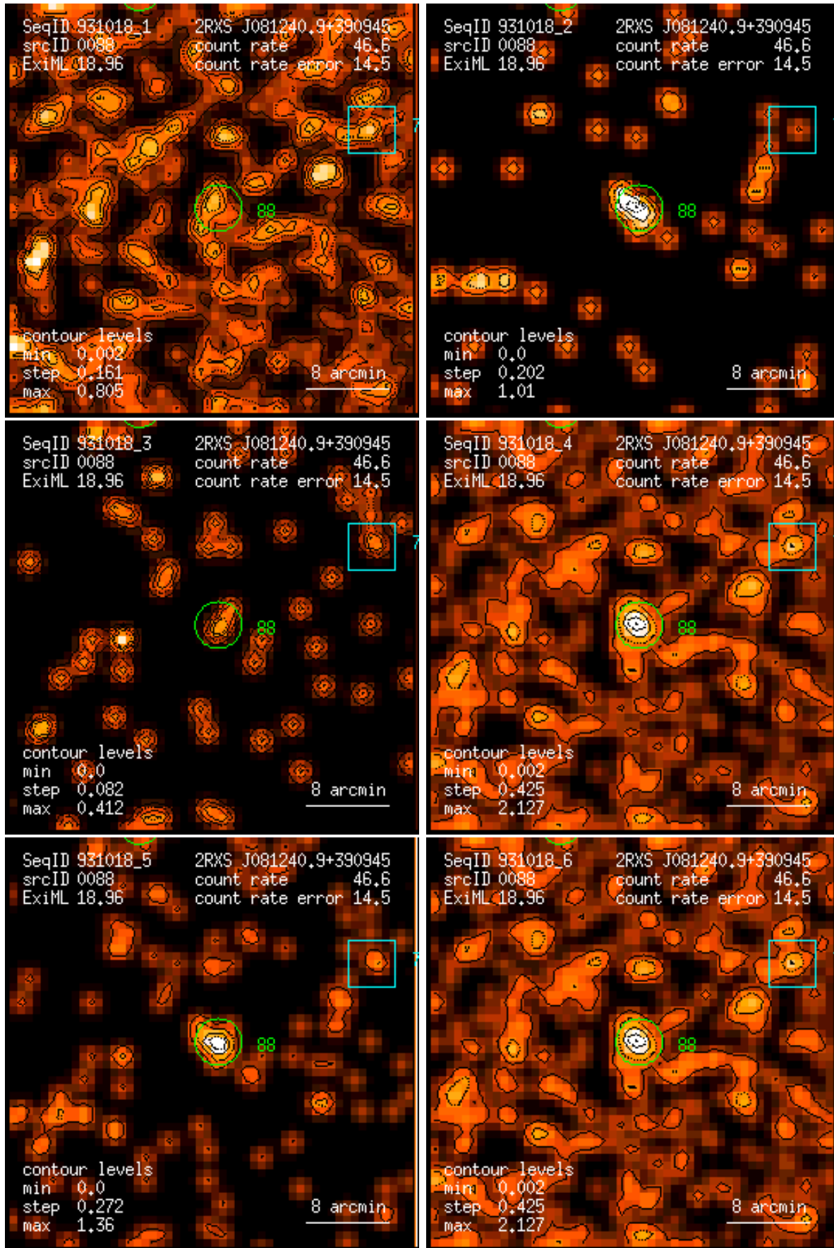
Figure 88: RASS 931018: detection 0088: band rate images, Gaussian filter: (1) PSPC channels 11 – 41, (2) 52 – 90, (3) 91 – 201, (4) 11 – 235, (5) 52 – 201, (6) 11 – 201. Broad band rates in counts/ks. Band rate contour levels in counts/ks/arcmin 2 .
