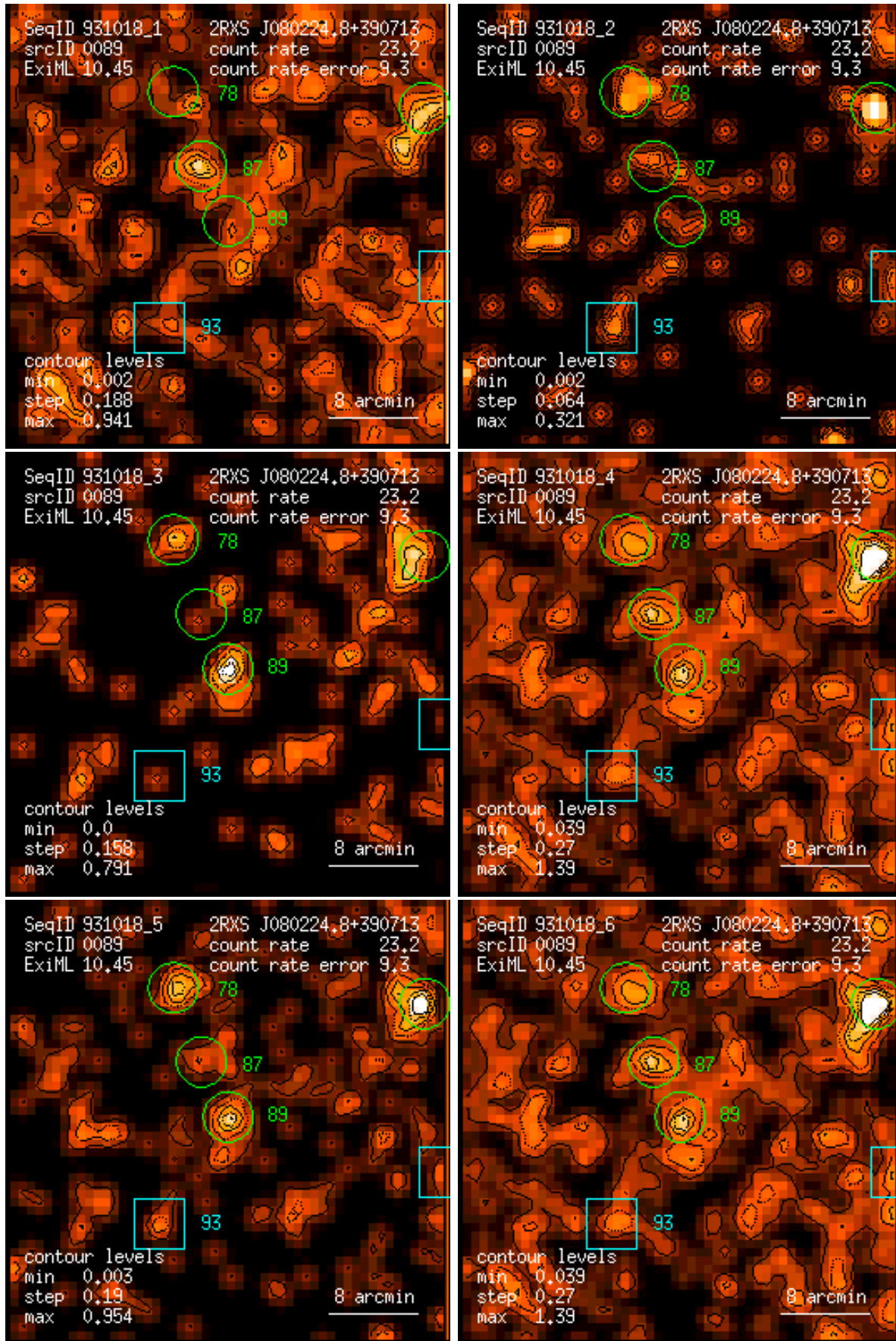
Figure 89: RASS 931018: detection 0089: band rate images, Gaussian filter: (1) PSPC channels 11 – 41, (2) 52 – 90, (3) 91 – 201, (4) 11 – 235, (5) 52 – 201, (6) 11 – 201. Broad band rates in counts/ks. Band rate contour levels in counts/ks/arcmin 2 .
