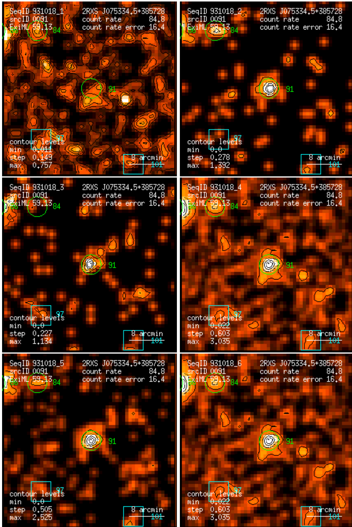
Figure 91: RASS 931018: detection 0091: band rate images, Gaussian filter: (1) PSPC channels 11 – 41, (2) 52 – 90, (3) 91 – 201, (4) 11 – 235, (5) 52 – 201, (6) 11 – 201. Broad band rates in counts/ks. Band rate contour levels in counts/ks/arcmin 2 .
