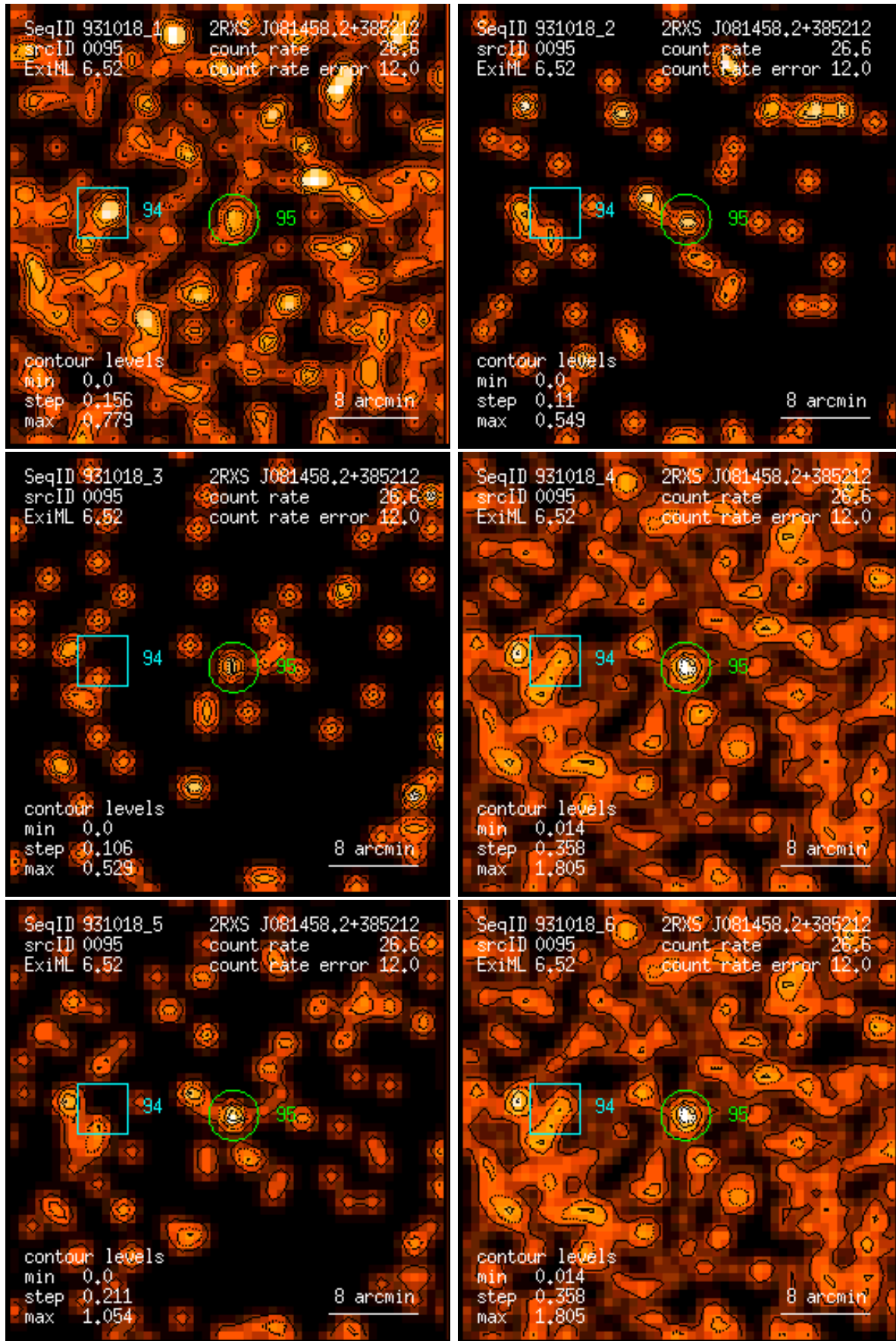
Figure 95: RASS 931018: detection 0095: band rate images, Gaussian filter: (1) PSPC channels 11 – 41, (2) 52 – 90, (3) 91 – 201, (4) 11 – 235, (5) 52 – 201, (6) 11 – 201. Broad band rates in counts/ks. Band rate contour levels in counts/ks/arcmin 2 .
