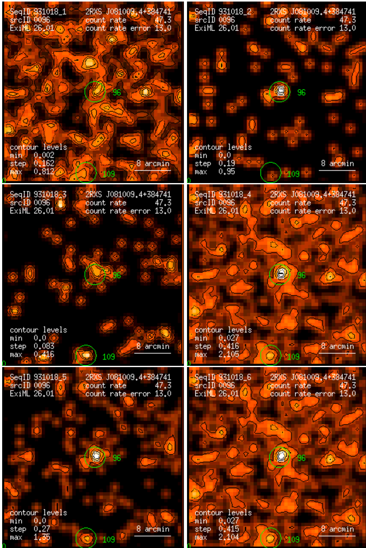
Figure 96: RASS 931018: detection 0096: band rate images, Gaussian filter: (1) PSPC channels 11 – 41, (2) 52 – 90, (3) 91 – 201, (4) 11 – 235, (5) 52 – 201, (6) 11 – 201. Broad band rates in counts/ks. Band rate contour levels in counts/ks/arcmin 2 .
