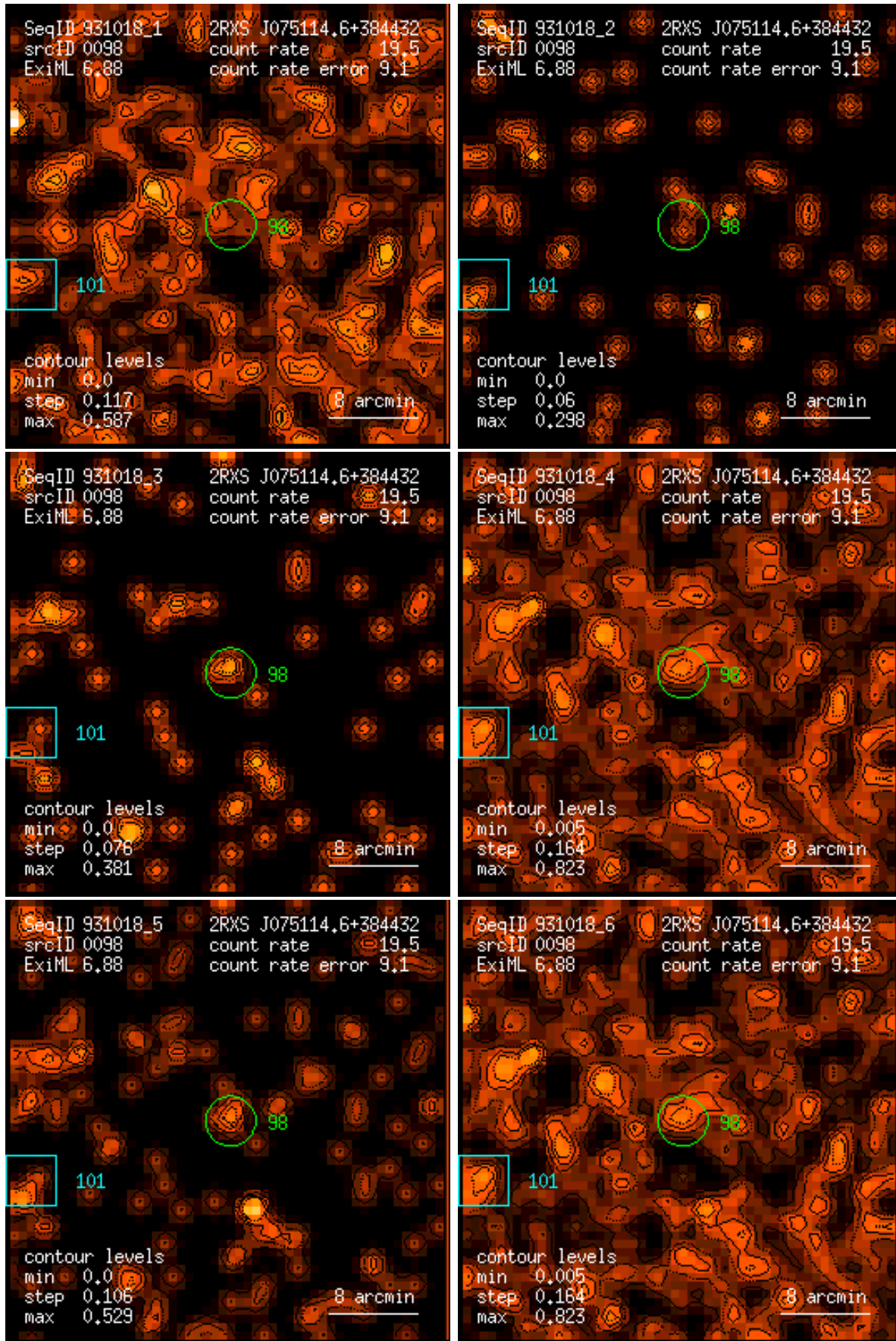
Figure 98: RASS 931018: detection 0098: band rate images, Gaussian filter: (1) PSPC channels 11 – 41, (2) 52 – 90, (3) 91 – 201, (4) 11 – 235, (5) 52 – 201, (6) 11 – 201. Broad band rates in counts/ks. Band rate contour levels in counts/ks/arcmin 2 .
