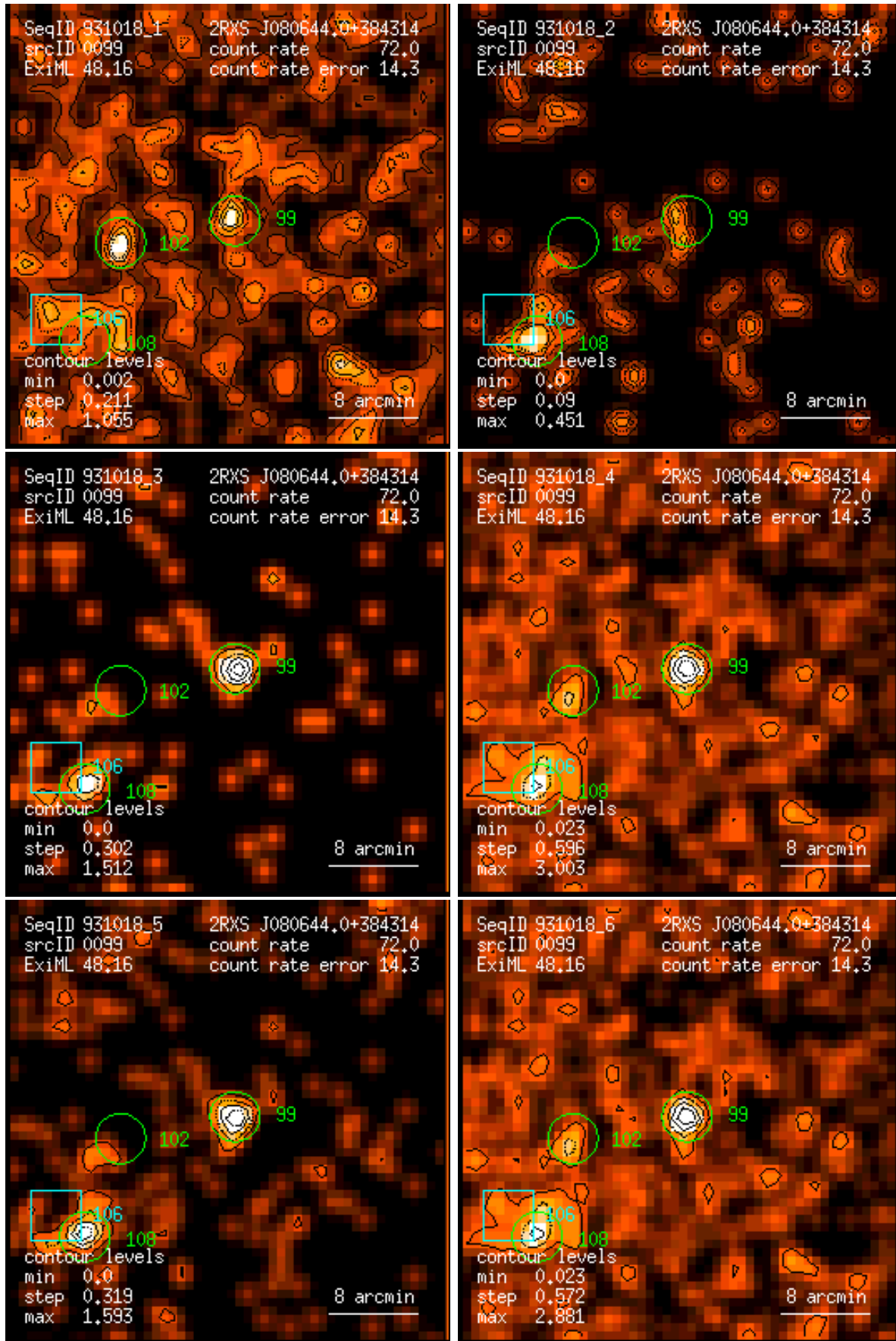
Figure 99: RASS 931018: detection 0099: band rate images, Gaussian filter: (1) PSPC channels 11 – 41, (2) 52 – 90, (3) 91 – 201, (4) 11 – 235, (5) 52 – 201, (6) 11 – 201. Broad band rates in counts/ks. Band rate contour levels in counts/ks/arcmin 2 .
