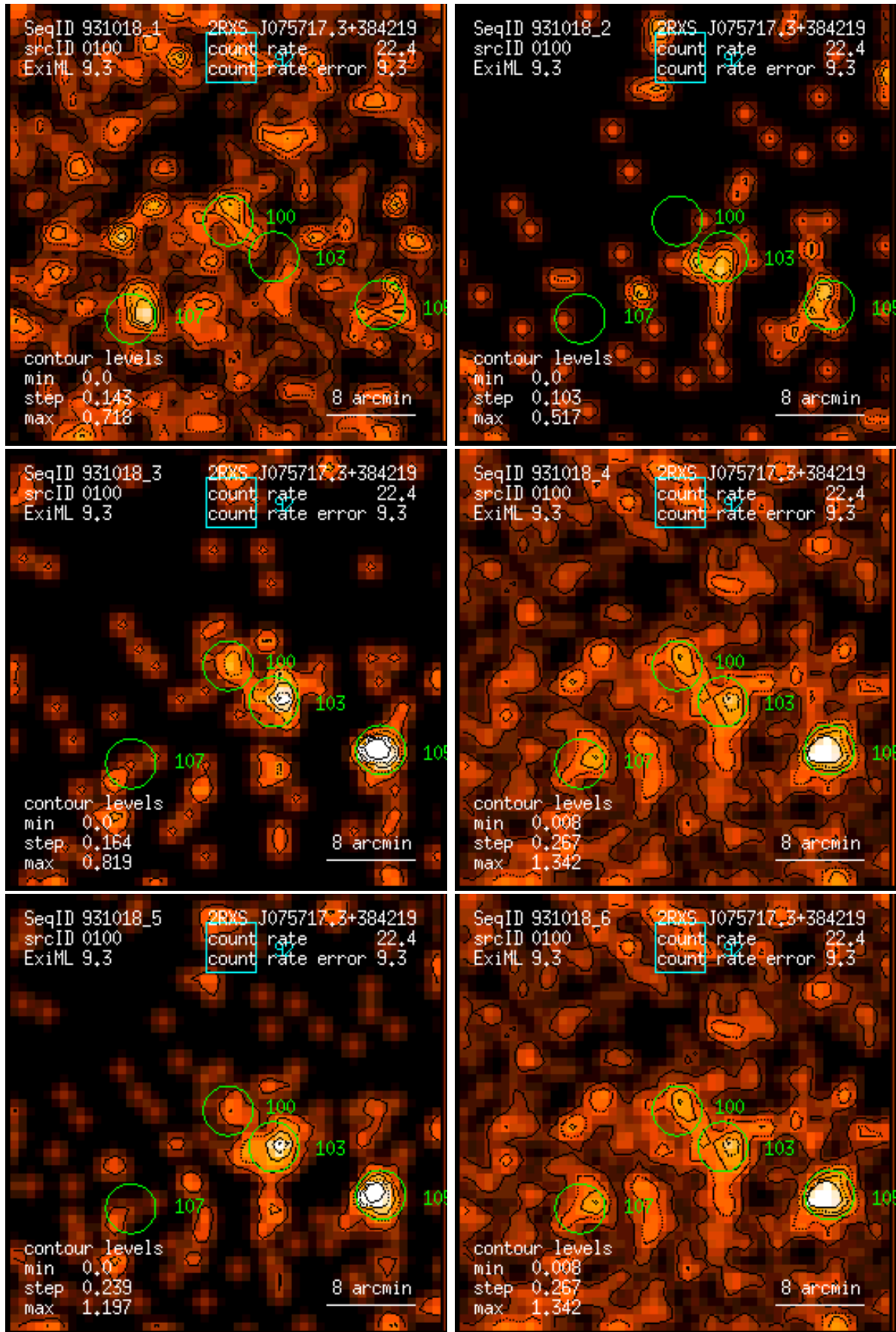
Figure 100: RASS 931018: detection 0100: band rate images, Gaussian filter: (1) PSPC channels 11 – 41, (2) 52 – 90, (3) 91 – 201, (4) 11 – 235, (5) 52 – 201, (6) 11 – 201. Broad band rates in counts/ks. Band rate contour levels in counts/ks/arcmin 2 .
