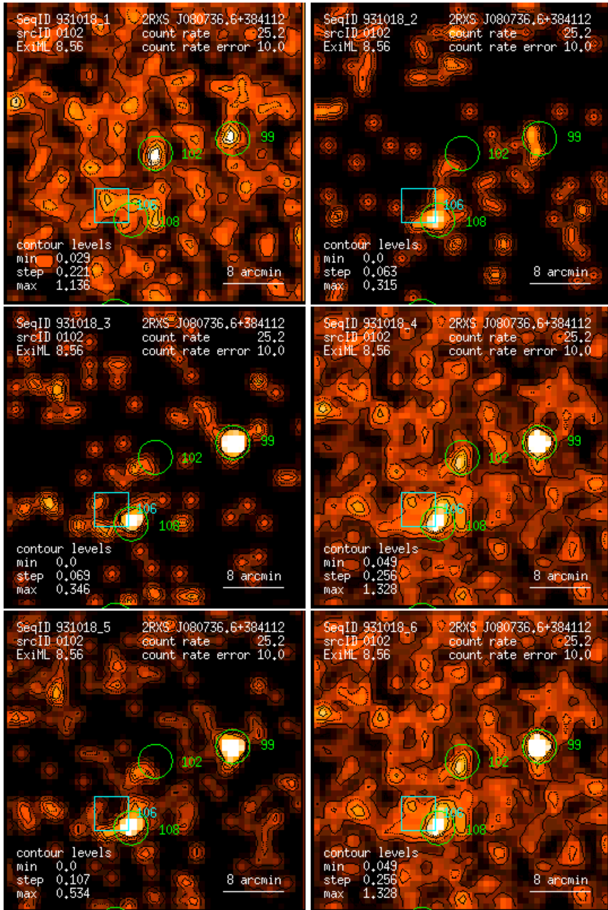
Figure 102: RASS 931018: detection 0102: band rate images, Gaussian filter: (1) PSPC channels 11 – 41, (2) 52 – 90, (3) 91 – 201, (4) 11 – 235, (5) 52 – 201, (6) 11 – 201. Broad band rates in counts/ks. Band rate contour levels in counts/ks/arcmin 2 .
