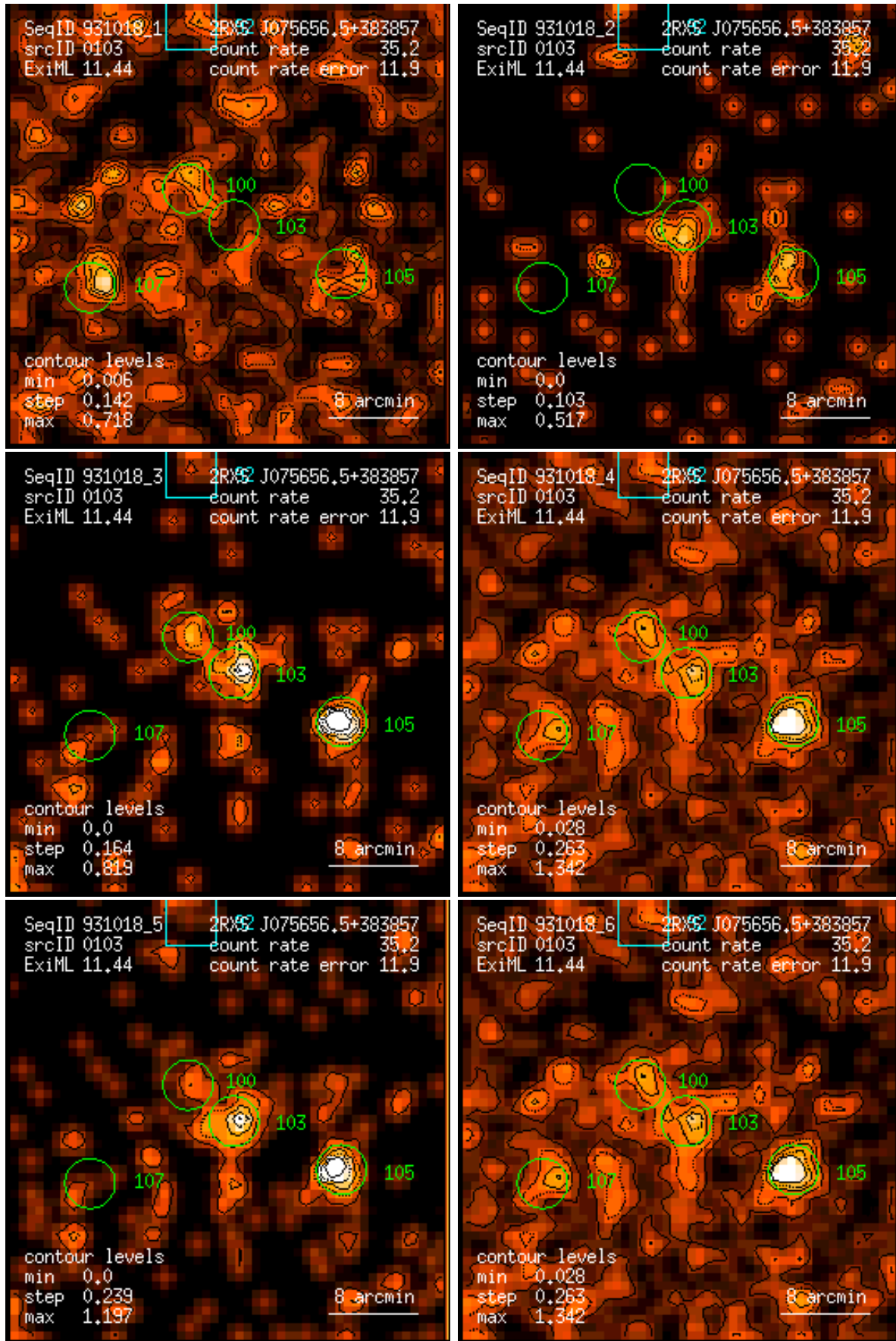
Figure 103: RASS 931018: detection 0103: band rate images, Gaussian filter: (1) PSPC channels 11 – 41, (2) 52 – 90, (3) 91 – 201, (4) 11 – 235, (5) 52 – 201, (6) 11 – 201. Broad band rates in counts/ks. Band rate contour levels in counts/ks/arcmin 2 .
