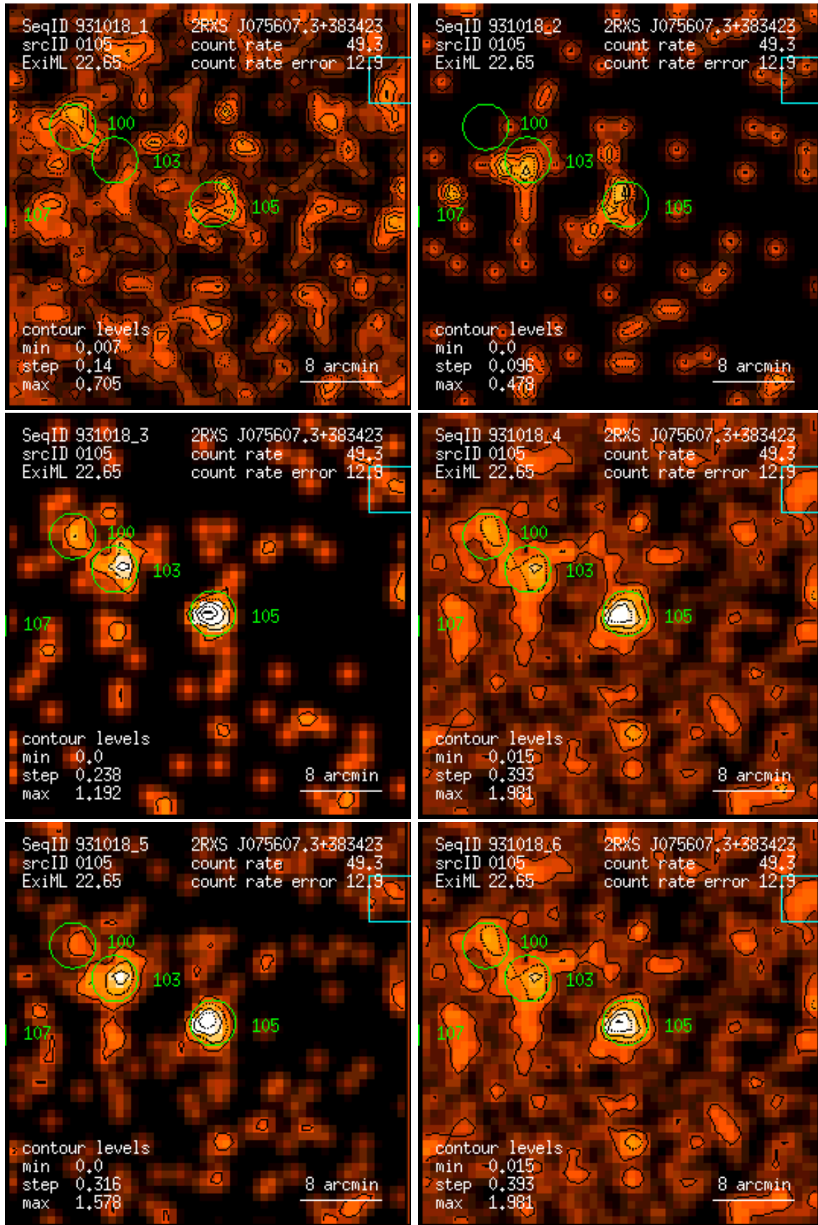
Figure 105: RASS 931018: detection 0105: band rate images, Gaussian filter: (1) PSPC channels 11 – 41, (2) 52 – 90, (3) 91 – 201, (4) 11 – 235, (5) 52 – 201, (6) 11 – 201. Broad band rates in counts/ks. Band rate contour levels in counts/ks/arcmin 2 .
