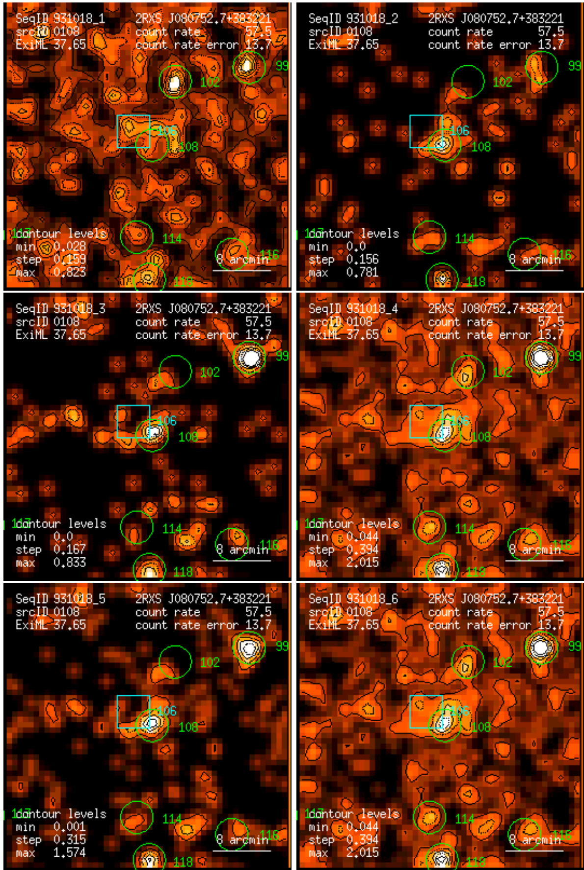
Figure 108: RASS 931018: detection 0108: band rate images, Gaussian filter: (1) PSPC channels 11 – 41, (2) 52 – 90, (3) 91 – 201, (4) 11 – 235, (5) 52 – 201, (6) 11 – 201. Broad band rates in counts/ks. Band rate contour levels in counts/ks/arcmin 2 .
