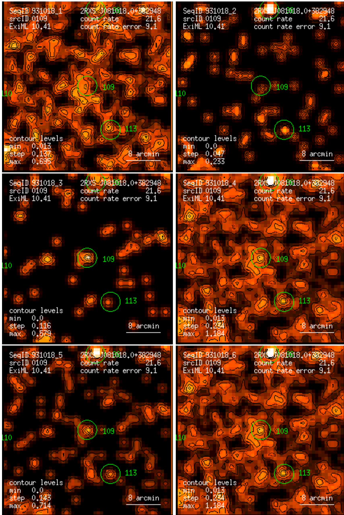
Figure 109: RASS 931018: detection 0109: band rate images, Gaussian filter: (1) PSPC channels 11 – 41, (2) 52 – 90, (3) 91 – 201, (4) 11 – 235, (5) 52 – 201, (6) 11 – 201. Broad band rates in counts/ks. Band rate contour levels in counts/ks/arcmin 2 .
