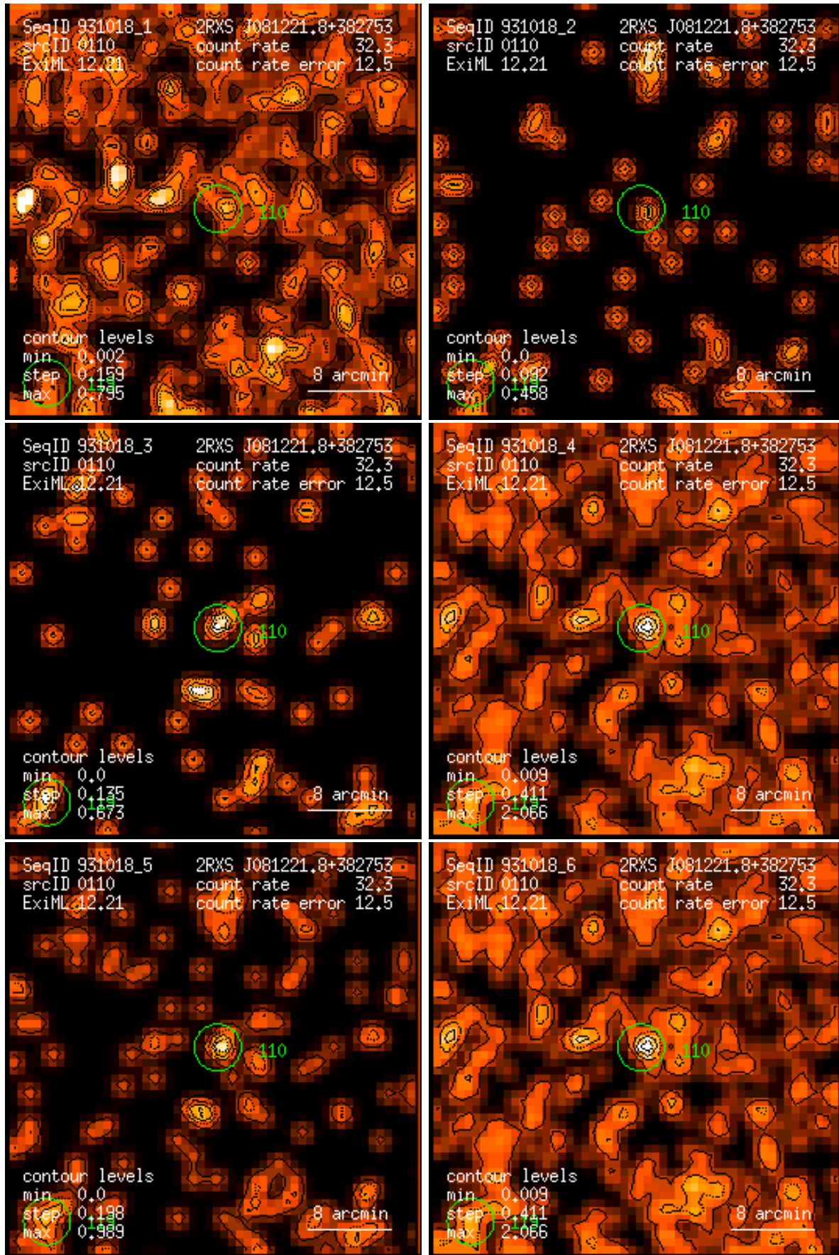
Figure 110: RASS 931018: detection 0110: band rate images, Gaussian filter: (1) PSPC channels 11 – 41, (2) 52 – 90, (3) 91 – 201, (4) 11 – 235, (5) 52 – 201, (6) 11 – 201. Broad band rates in counts/ks. Band rate contour levels in counts/ks/arcmin 2 .
