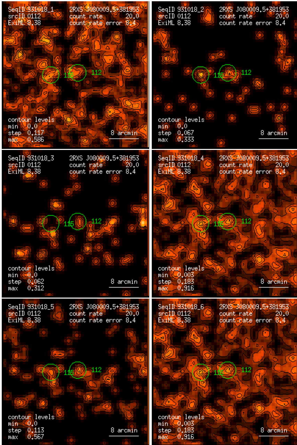
Figure 112: RASS 931018: detection 0112: band rate images, Gaussian filter: (1) PSPC channels 11 – 41, (2) 52 – 90, (3) 91 – 201, (4) 11 – 235, (5) 52 – 201, (6) 11 – 201. Broad band rates in counts/ks. Band rate contour levels in counts/ks/arcmin 2 .
