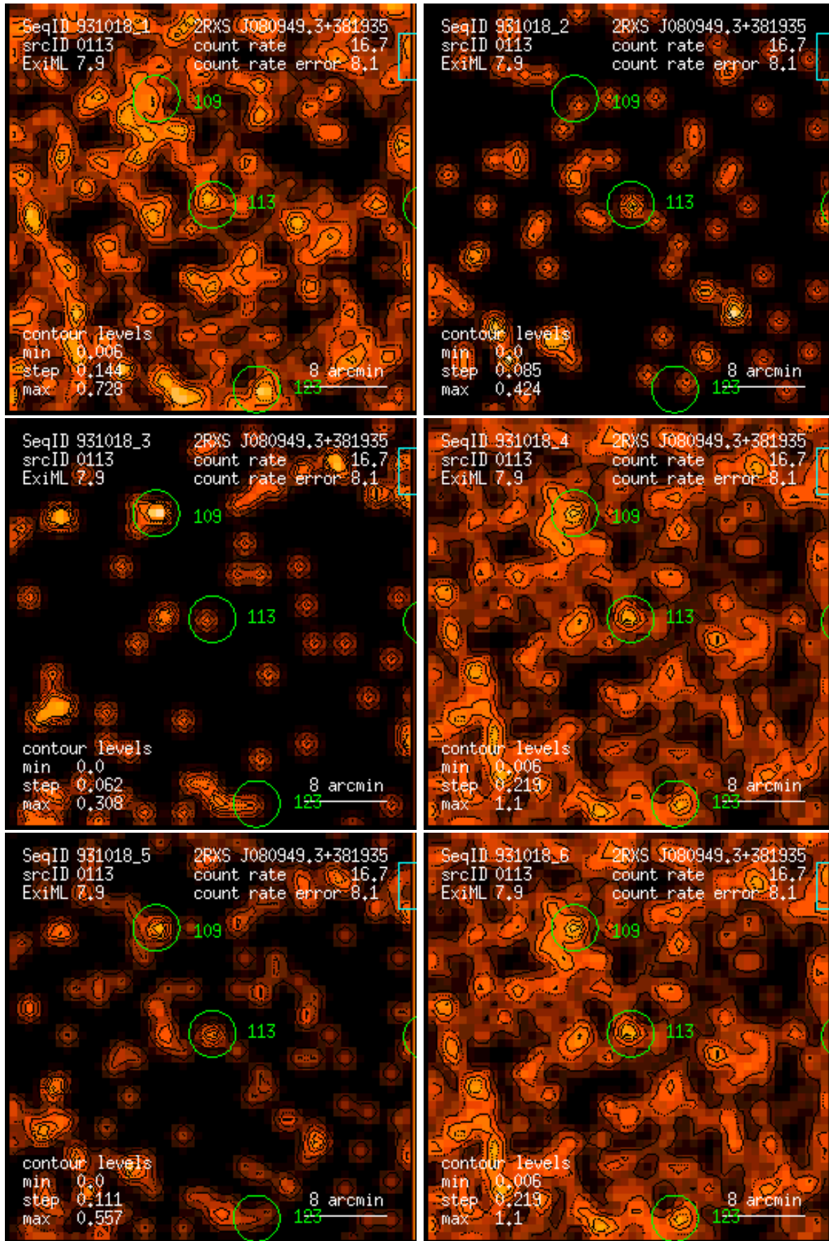
Figure 113: RASS 931018: detection 0113: band rate images, Gaussian filter: (1) PSPC channels 11 – 41, (2) 52 – 90, (3) 91 – 201, (4) 11 – 235, (5) 52 – 201, (6) 11 – 201. Broad band rates in counts/ks. Band rate contour levels in counts/ks/arcmin 2 .
