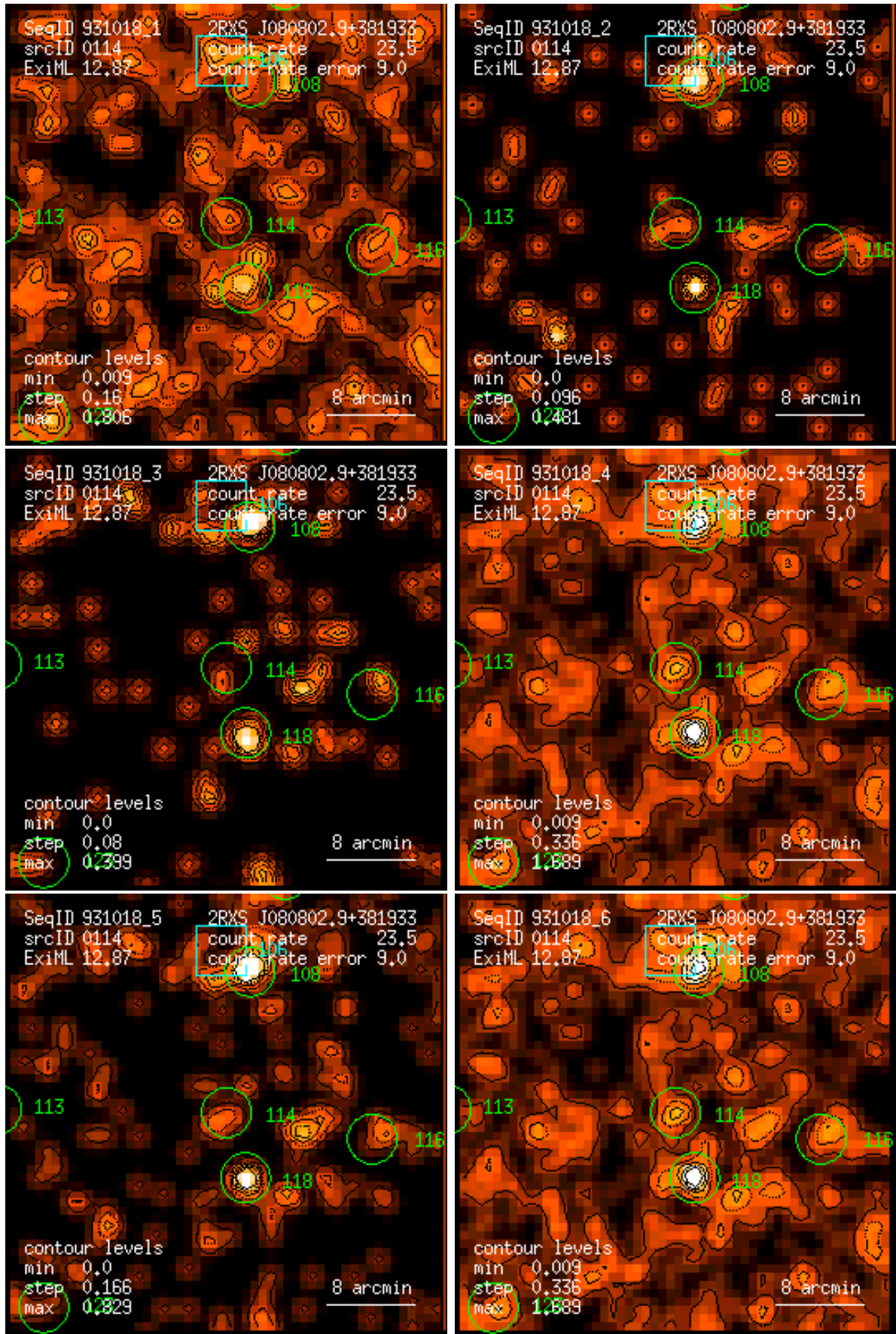
Figure 114: RASS 931018: detection 0114: band rate images, Gaussian filter: (1) PSPC channels 11 – 41, (2) 52 – 90, (3) 91 – 201, (4) 11 – 235, (5) 52 – 201, (6) 11 – 201. Broad band rates in counts/ks. Band rate contour levels in counts/ks/arcmin 2 .
