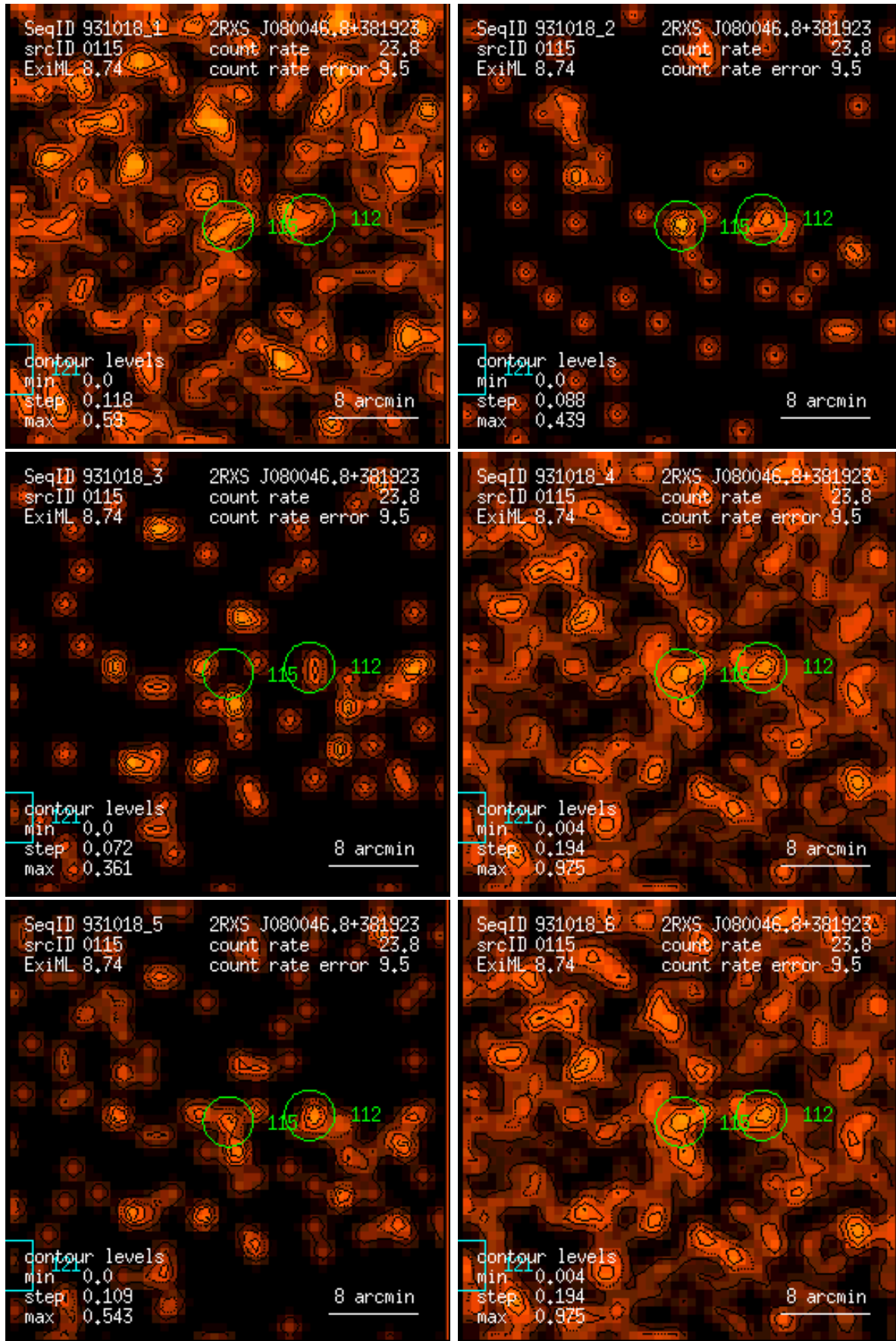
Figure 115: RASS 931018: detection 0115: band rate images, Gaussian filter: (1) PSPC channels 11 – 41, (2) 52 – 90, (3) 91 – 201, (4) 11 – 235, (5) 52 – 201, (6) 11 – 201. Broad band rates in counts/ks. Band rate contour levels in counts/ks/arcmin 2 .
