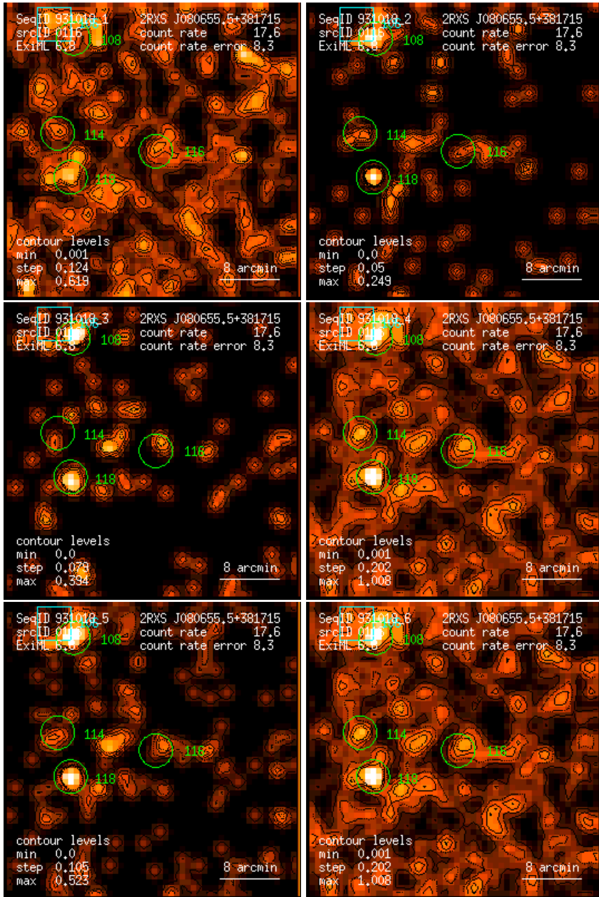
Figure 116: RASS 931018: detection 0116: band rate images, Gaussian filter: (1) PSPC channels 11 – 41, (2) 52 – 90, (3) 91 – 201, (4) 11 – 235, (5) 52 – 201, (6) 11 – 201. Broad band rates in counts/ks. Band rate contour levels in counts/ks/arcmin 2 .
