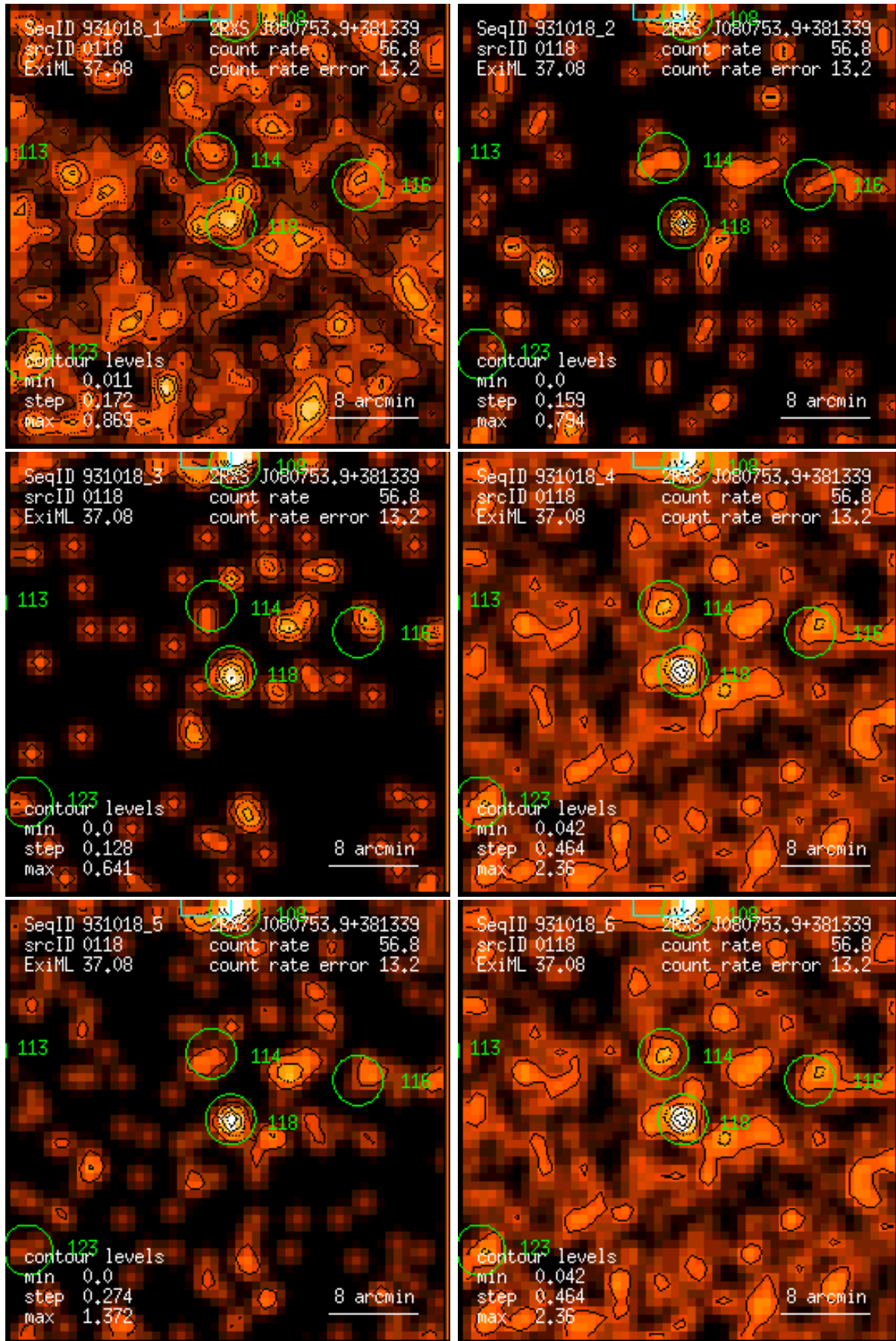
Figure 118: RASS 931018: detection 0118: band rate images, Gaussian filter: (1) PSPC channels 11 – 41, (2) 52 – 90, (3) 91 – 201, (4) 11 – 235, (5) 52 – 201, (6) 11 – 201. Broad band rates in counts/ks. Band rate contour levels in counts/ks/arcmin 2 .
