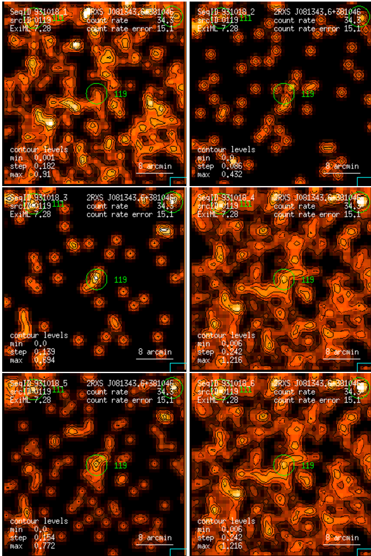
Figure 119: RASS 931018: detection 0119: band rate images, Gaussian filter: (1) PSPC channels 11 – 41, (2) 52 – 90, (3) 91 – 201, (4) 11 – 235, (5) 52 – 201, (6) 11 – 201. Broad band rates in counts/ks. Band rate contour levels in counts/ks/arcmin 2 .
