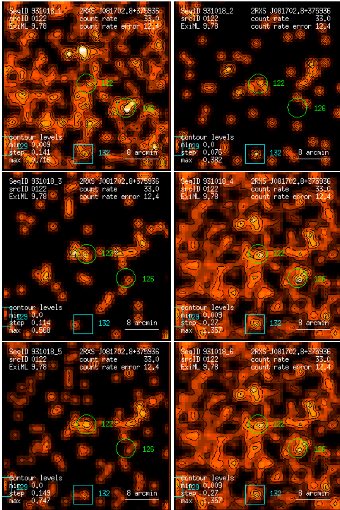
Figure 122: RASS 931018: detection 0122: band rate images, Gaussian filter: (1) PSPC channels 11 – 41, (2) 52 – 90, (3) 91 – 201, (4) 11 – 235, (5) 52 – 201, (6) 11 – 201. Broad band rates in counts/ks. Band rate contour levels in counts/ks/arcmin 2 .
