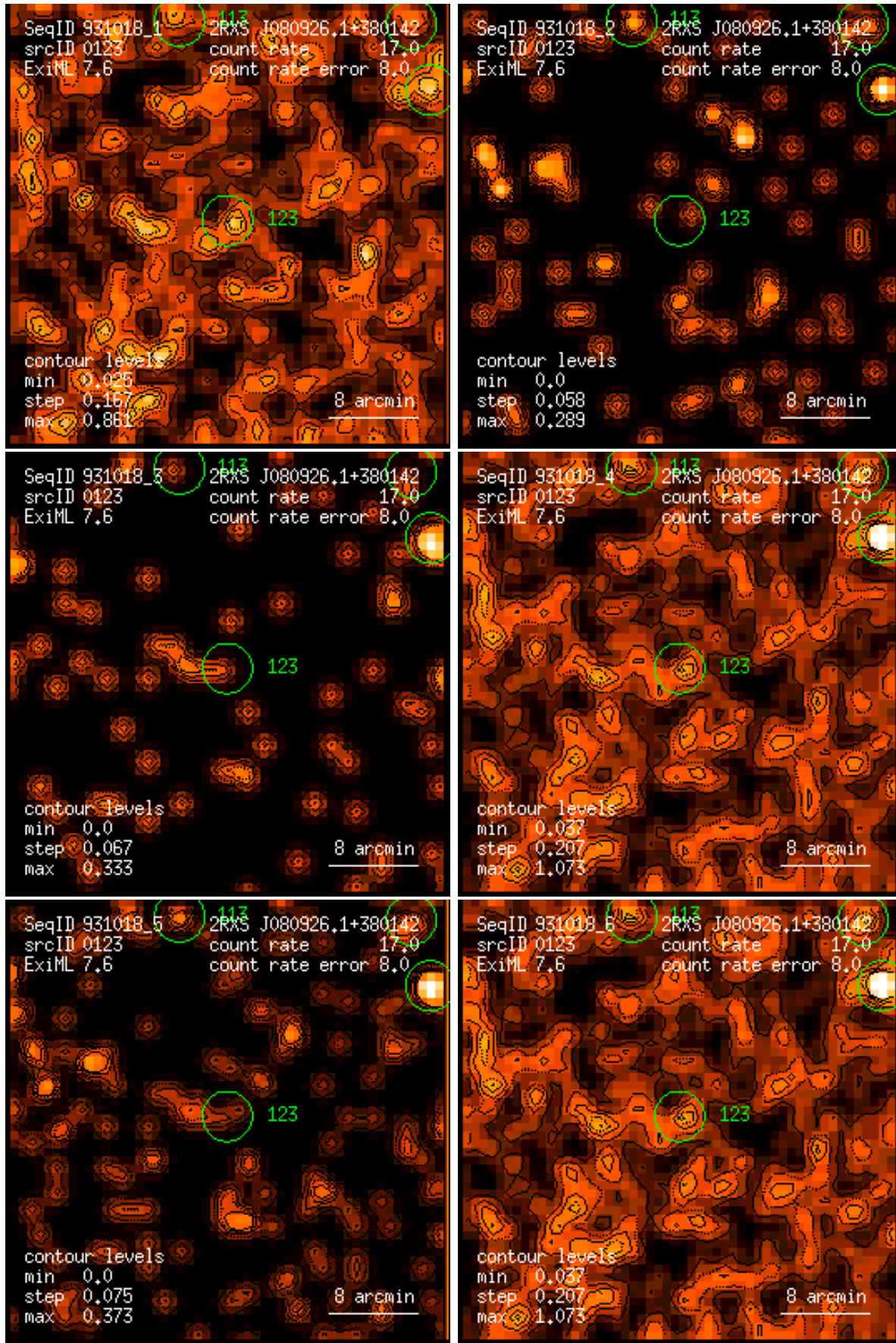
Figure 123: RASS 931018: detection 0123: band rate images, Gaussian filter: (1) PSPC channels 11 – 41, (2) 52 – 90, (3) 91 – 201, (4) 11 – 235, (5) 52 – 201, (6) 11 – 201. Broad band rates in counts/ks. Band rate contour levels in counts/ks/arcmin 2 .
