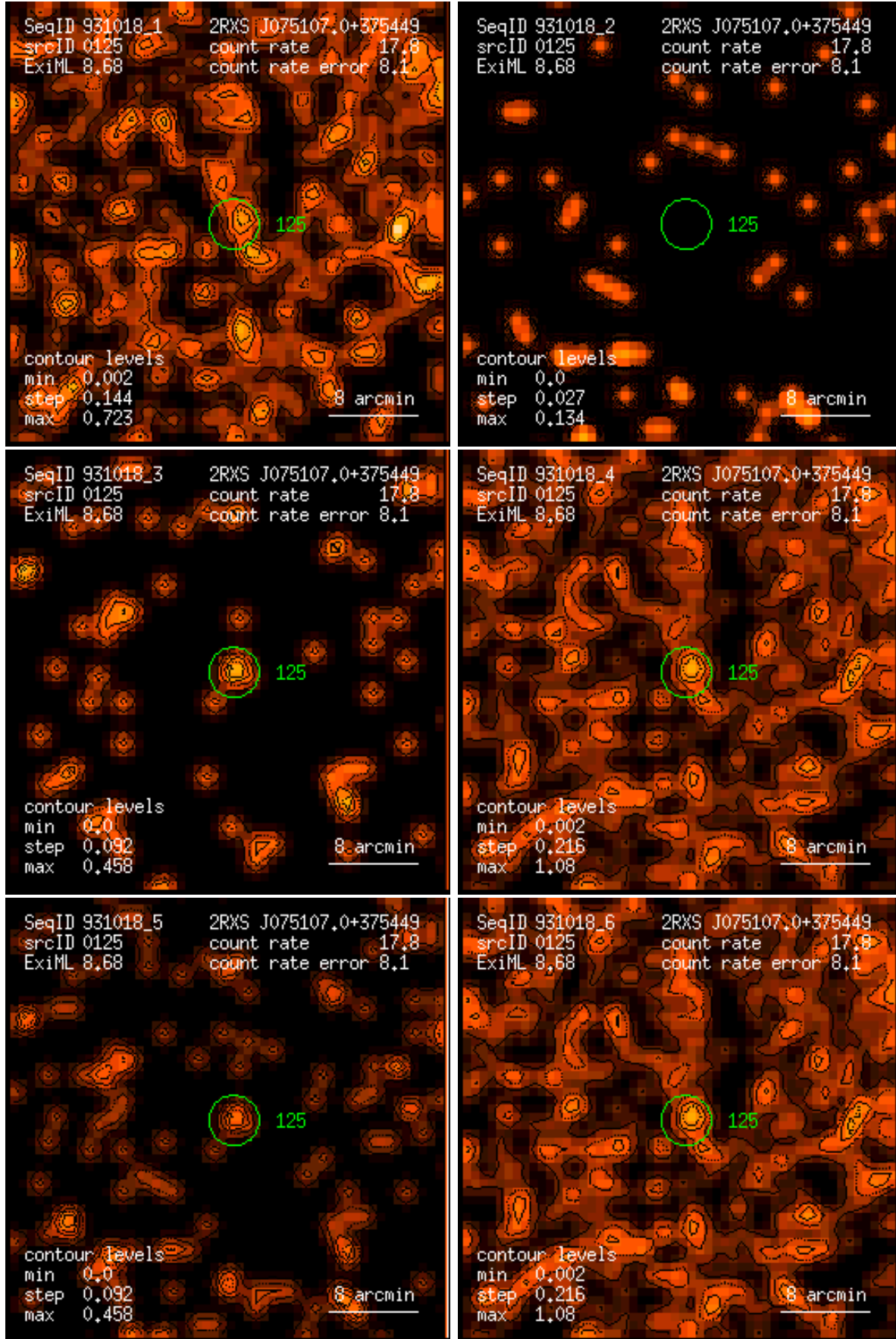
Figure 125: RASS 931018: detection 0125: band rate images, Gaussian filter: (1) PSPC channels 11 – 41, (2) 52 – 90, (3) 91 – 201, (4) 11 – 235, (5) 52 – 201, (6) 11 – 201. Broad band rates in counts/ks. Band rate contour levels in counts/ks/arcmin 2 .
