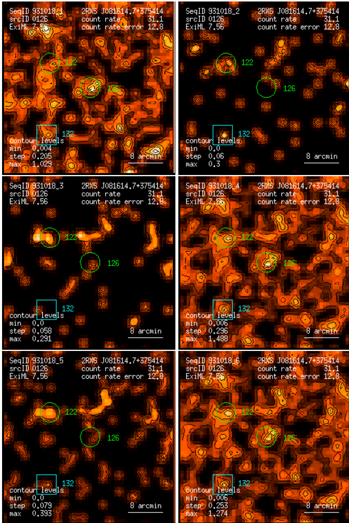
Figure 126: RASS 931018: detection 0126: band rate images, Gaussian filter: (1) PSPC channels 11 – 41, (2) 52 – 90, (3) 91 – 201, (4) 11 – 235, (5) 52 – 201, (6) 11 – 201. Broad band rates in counts/ks. Band rate contour levels in counts/ks/arcmin 2 .
