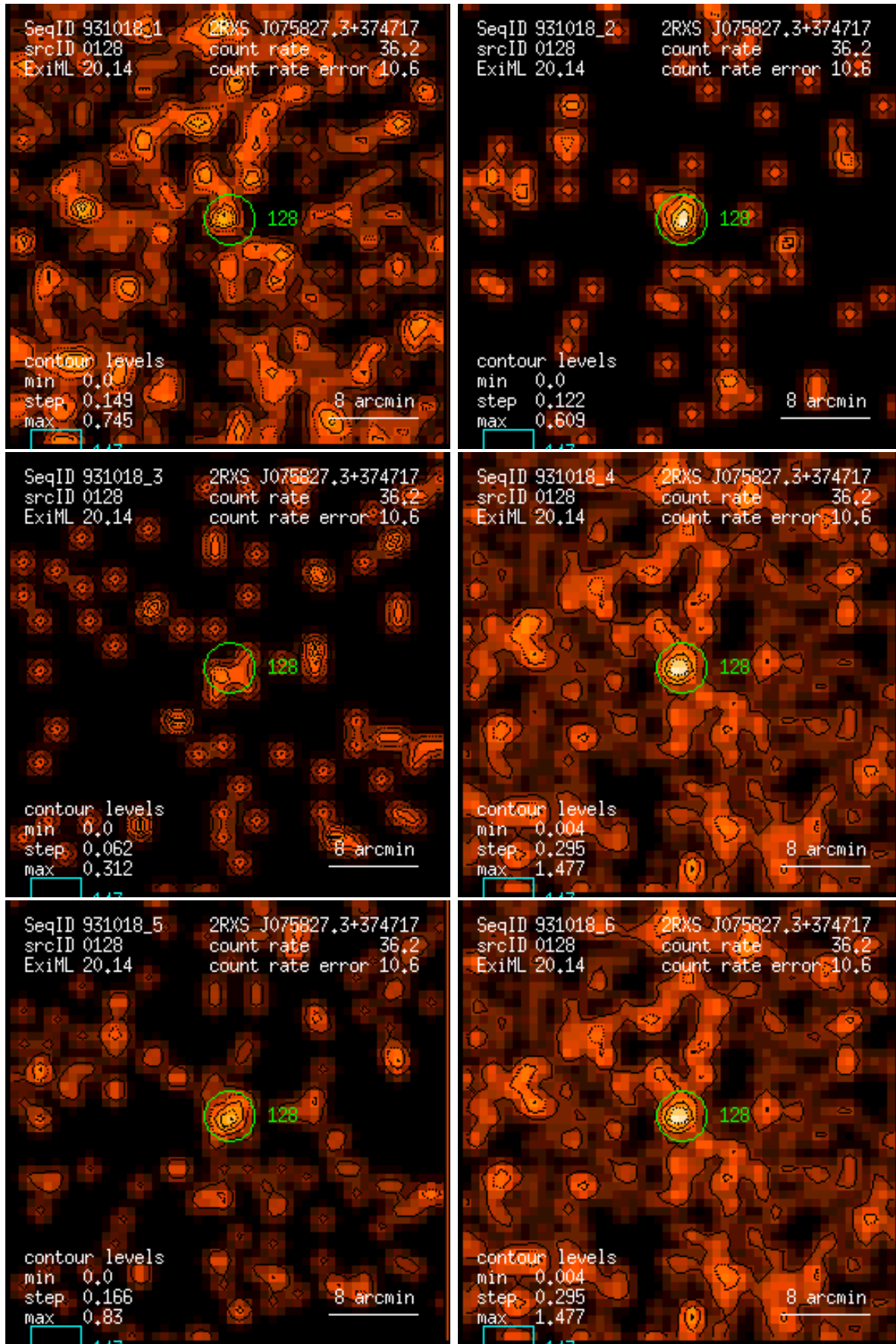
Figure 128: RASS 931018: detection 0128: band rate images, Gaussian filter: (1) PSPC channels 11 – 41, (2) 52 – 90, (3) 91 – 201, (4) 11 – 235, (5) 52 – 201, (6) 11 – 201. Broad band rates in counts/ks. Band rate contour levels in counts/ks/arcmin 2 .
