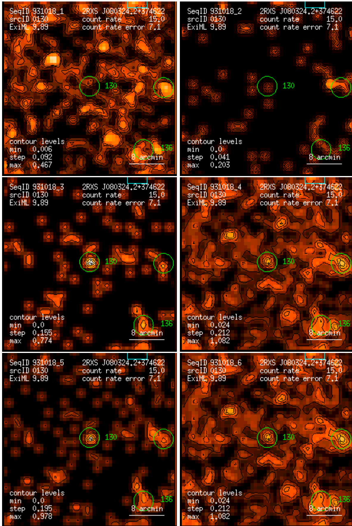
Figure 130: RASS 931018: detection 0130: band rate images, Gaussian filter: (1) PSPPC channels 11 – 41, (2) 52 – 90, (3) 91 – 201, (4) 11 – 235, (5) 52 – 201, (6) 11 – 201. Broad band rates in counts/ks. Band rate contour levels in counts/ks/arcmin 2 .
