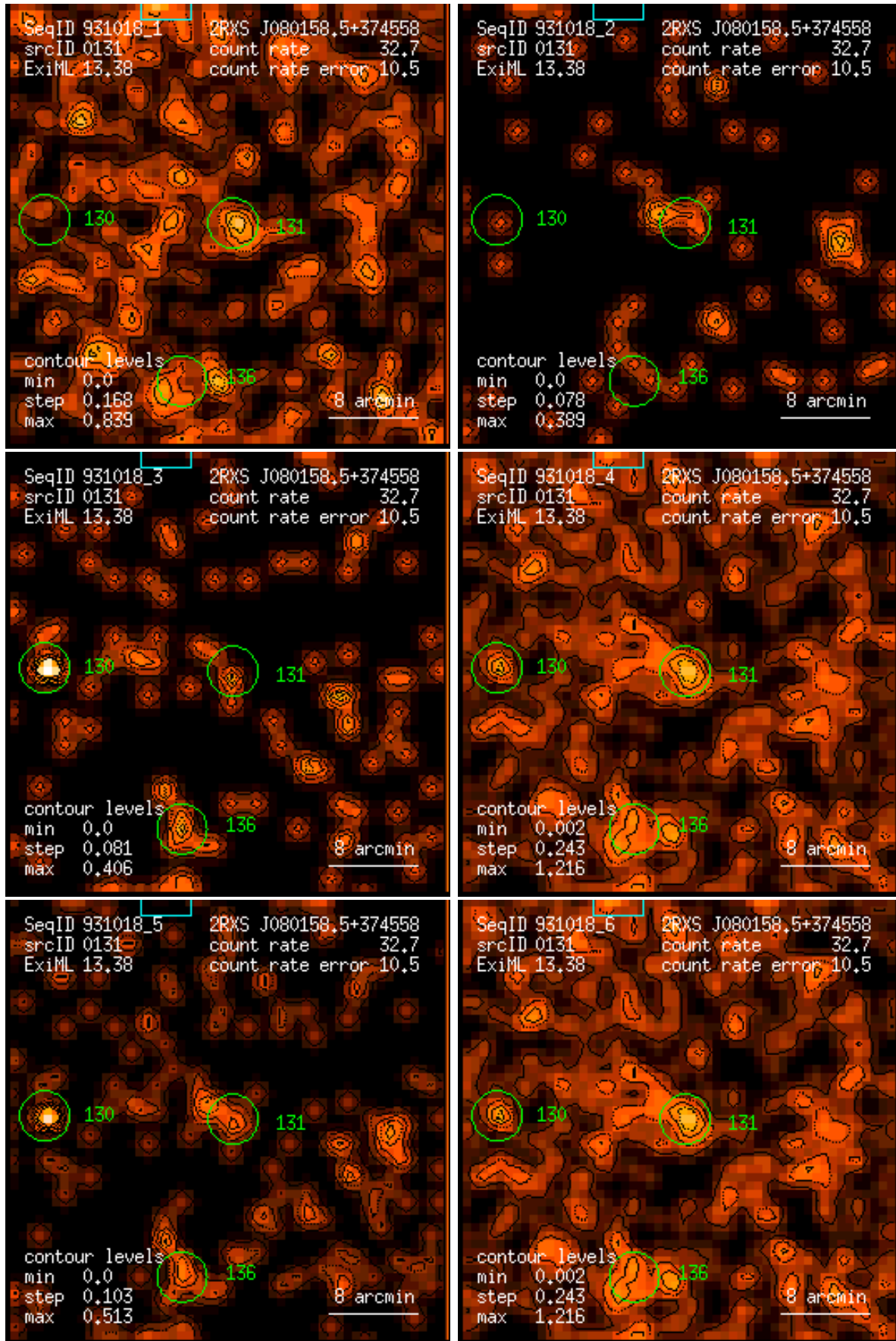
Figure 131: RASS 931018: detection 0131: band rate images, Gaussian filter: (1) PSPC channels 11 – 41, (2) 52 – 90, (3) 91 – 201, (4) 11 – 235, (5) 52 – 201, (6) 11 – 201. Broad band rates in counts/ks. Band rate contour levels in counts/ks/arcmin 2 .
