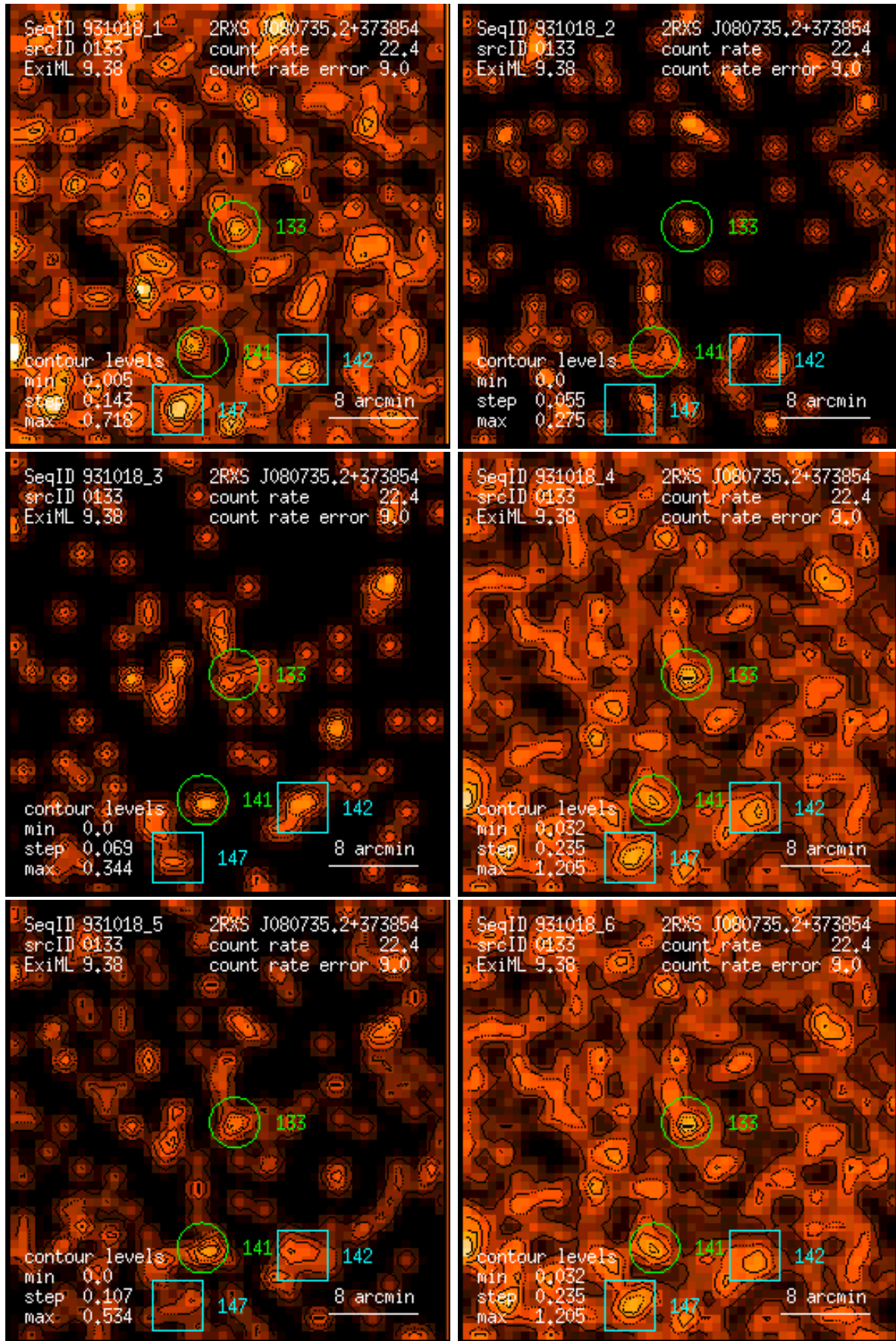
Figure 133: RASS 931018: detection 0133: band rate images, Gaussian filter: (1) PSPC channels 11 – 41, (2) 52 – 90, (3) 91 – 201, (4) 11 – 235, (5) 52 – 201, (6) 11 – 201. Broad band rates in counts/ks. Band rate contour levels in counts/ks/arcmin 2 .
