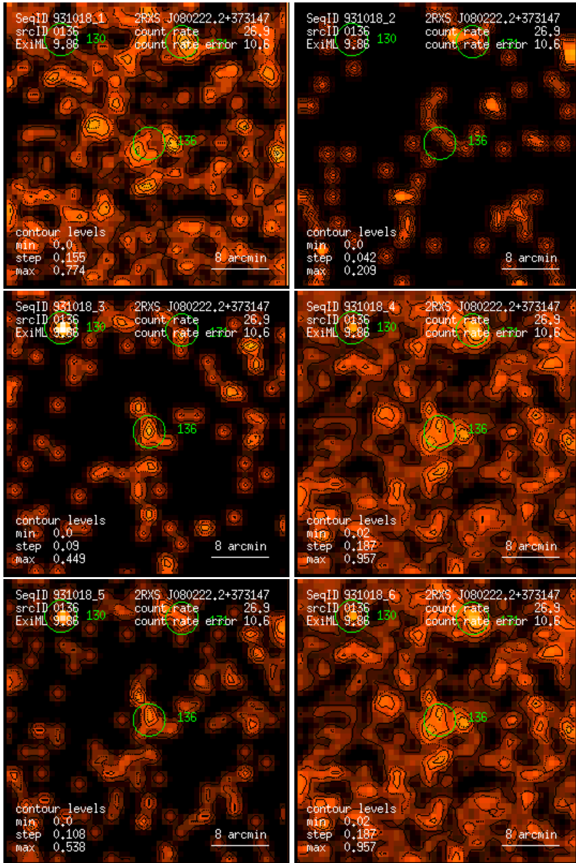
Figure 136: RASS 931018: detection 0136: band rate images, Gaussian filter: (1) PSPC channels 11 – 41, (2) 52 – 90, (3) 91 – 201, (4) 11 – 235, (5) 52 – 201, (6) 11 – 201. Broad band rates in counts/ks. Band rate contour levels in counts/ks/arcmin 2 .
