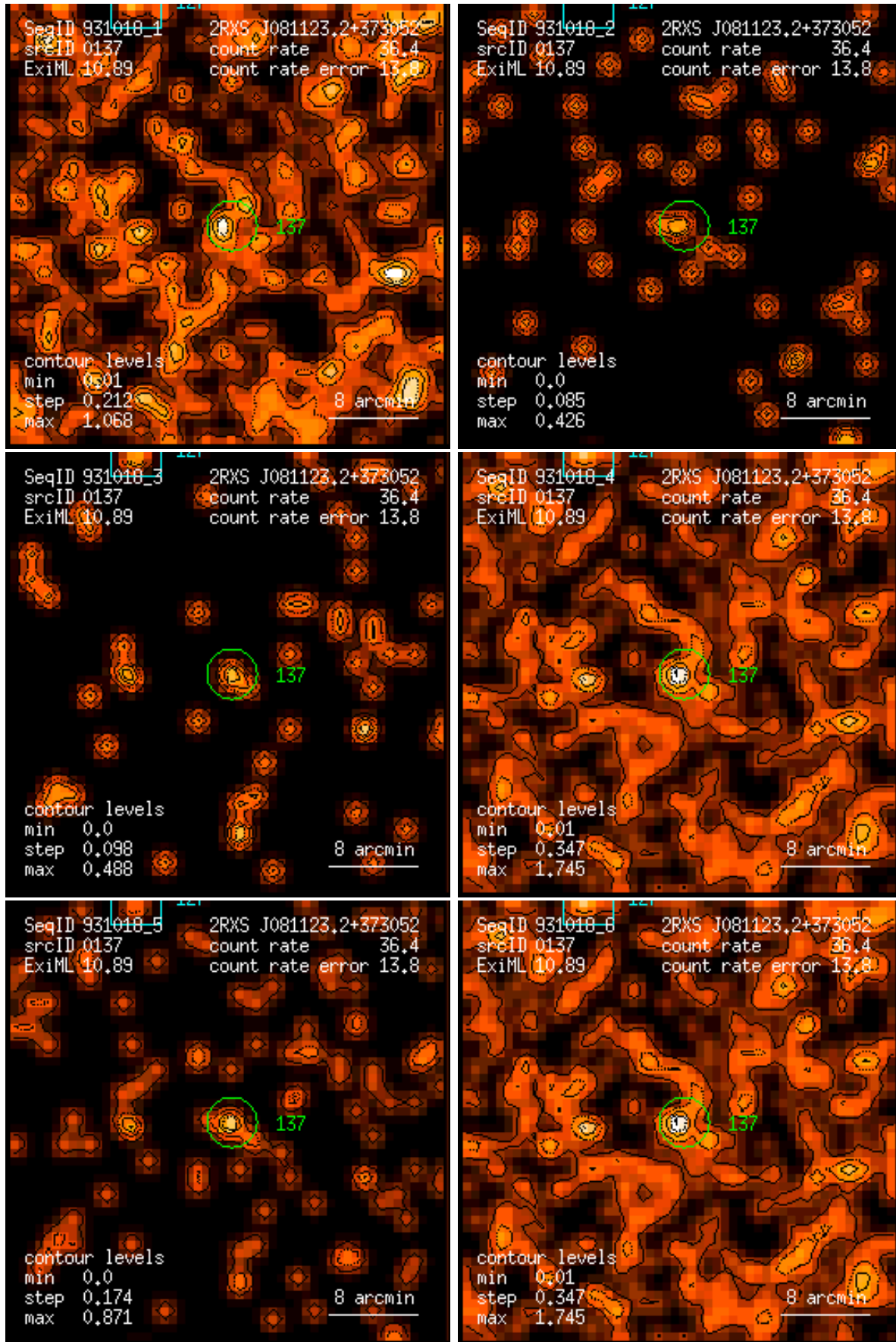
Figure 137: RASS 931018: detection 0137: band rate images, Gaussian filter: (1) PSPC channels 11 – 41, (2) 52 – 90, (3) 91 – 201, (4) 11 – 235, (5) 52 – 201, (6) 11 – 201. Broad band rates in counts/ks. Band rate contour levels in counts/ks/arcmin 2 .
