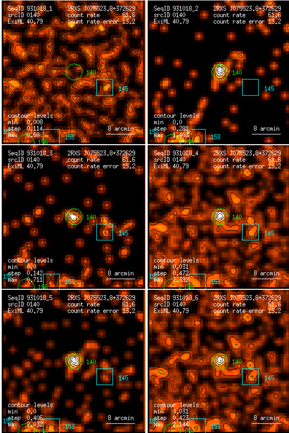
Figure 140: RASS 931018: detection 0140: band rate images, Gaussian filter: (1) PSPC channels 11 – 41, (2) 52 – 90, (3) 91 – 201, (4) 11 – 235, (5) 52 – 201, (6) 11 – 201. Broad band rates in counts/ks. Band rate contour levels in counts/ks/arcmin 2 .
