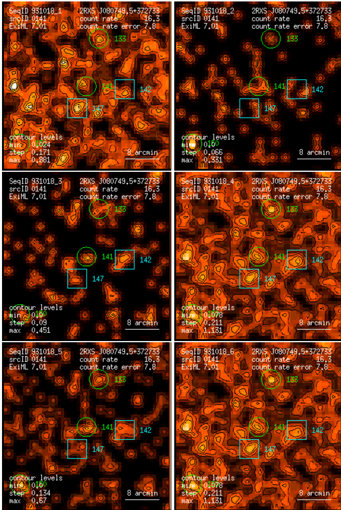
Figure 141: RASS 931018: detection 0141: band rate images, Gaussian filter: (1) PSPC channels 11 – 41, (2) 52 – 90, (3) 91 – 201, (4) 11 – 235, (5) 52 – 201, (6) 11 – 201. Broad band rates in counts/ks. Band rate contour levels in counts/ks/arcmin 2 .
