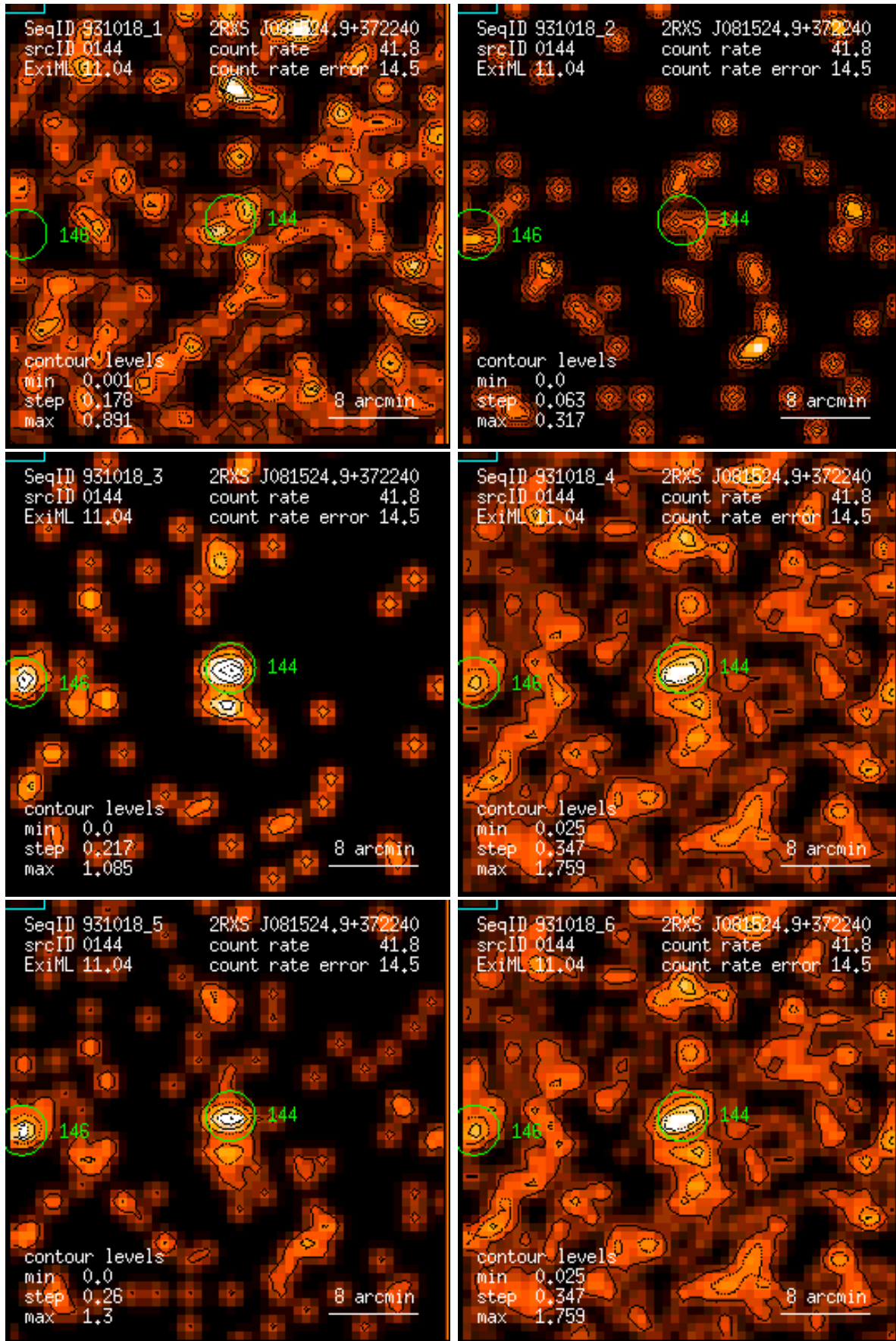
Figure 144: RASS 931018: detection 0144: band rate images, Gaussian filter: (1) PSPC channels 11 – 41, (2) 52 – 90, (3) 91 – 201, (4) 11 – 235, (5) 52 – 201, (6) 11 – 201. Broad band rates in counts/ks. Band rate contour levels in counts/ks/arcmin 2 .
