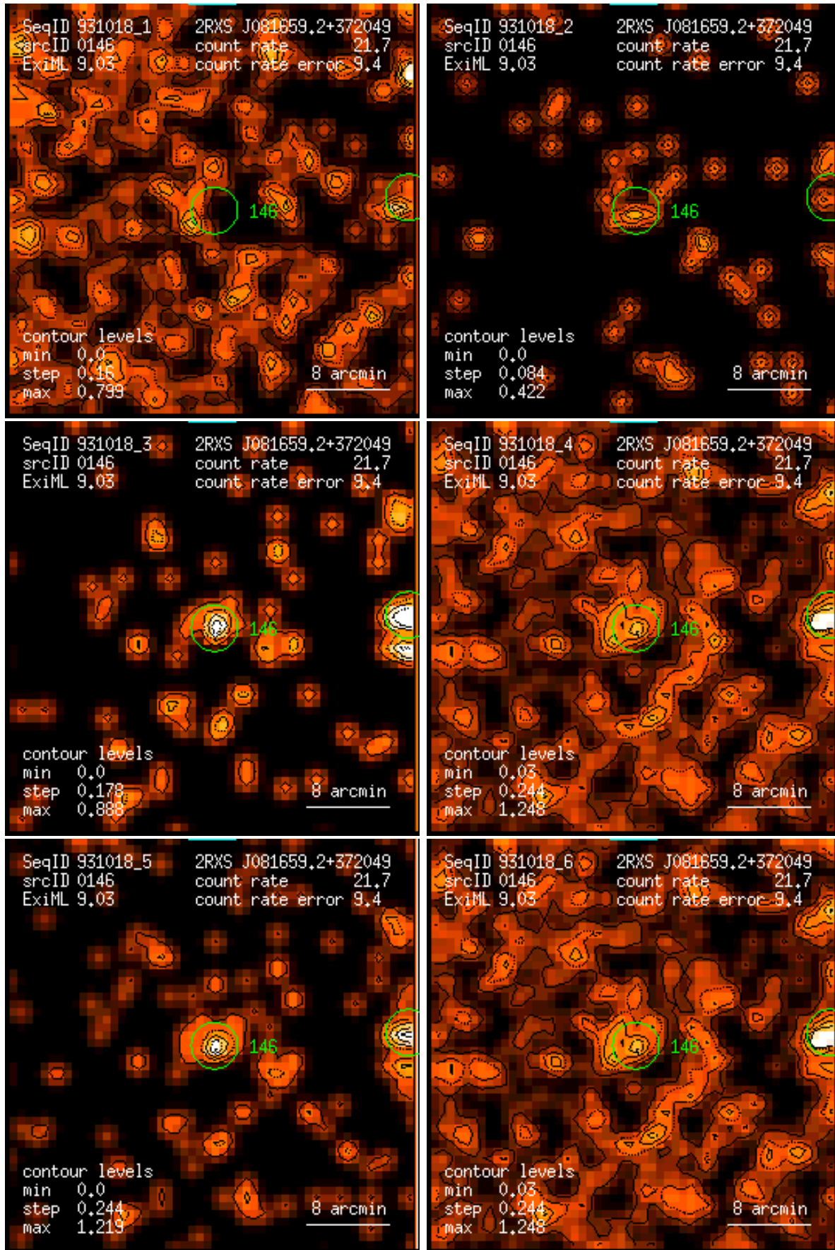
Figure 146: RASS 931018: detection 0146: band rate images, Gaussian filter: (1) PSPC channels 11 – 41, (2) 52 – 90, (3) 91 – 201, (4) 11 – 235, (5) 52 – 201, (6) 11 – 201. Broad band rates in counts/ks. Band rate contour levels in counts/ks/arcmin 2 .
