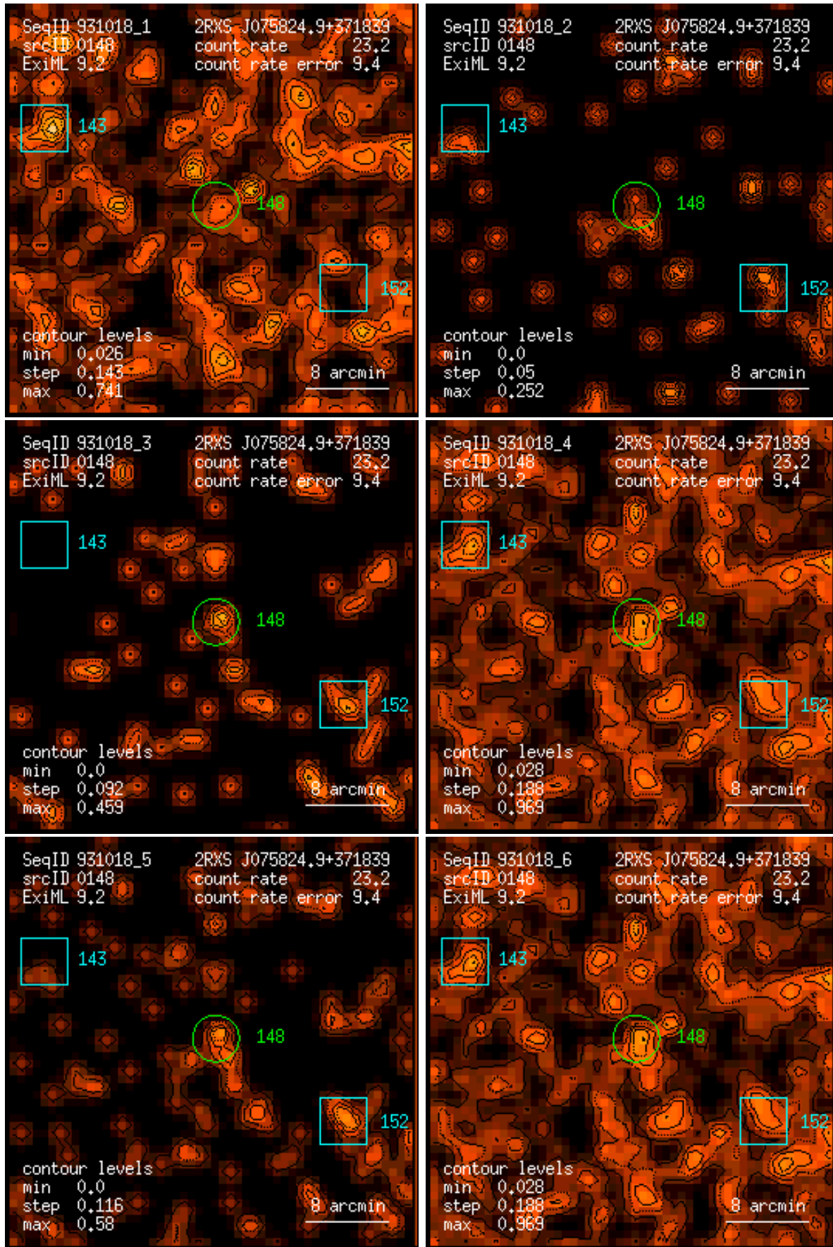
Figure 148: RASS 931018: detection 0148: band rate images, Gaussian filter: (1) PSPC channels 11 – 41, (2) 52 – 90, (3) 91 – 201, (4) 11 – 235, (5) 52 – 201, (6) 11 – 201. Broad band rates in counts/ks. Band rate contour levels in counts/ks/arcmin 2 .
